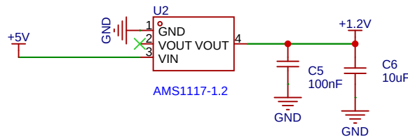
5V-1.2V LDO
