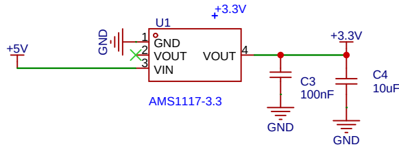
5V-3.3V LDO
