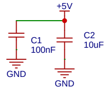
POWER IN
