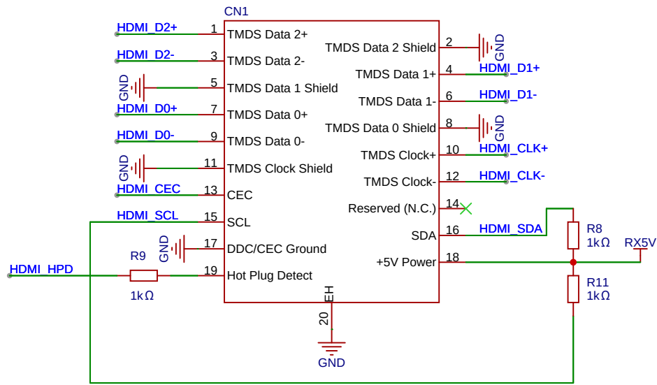
HDMI IN
