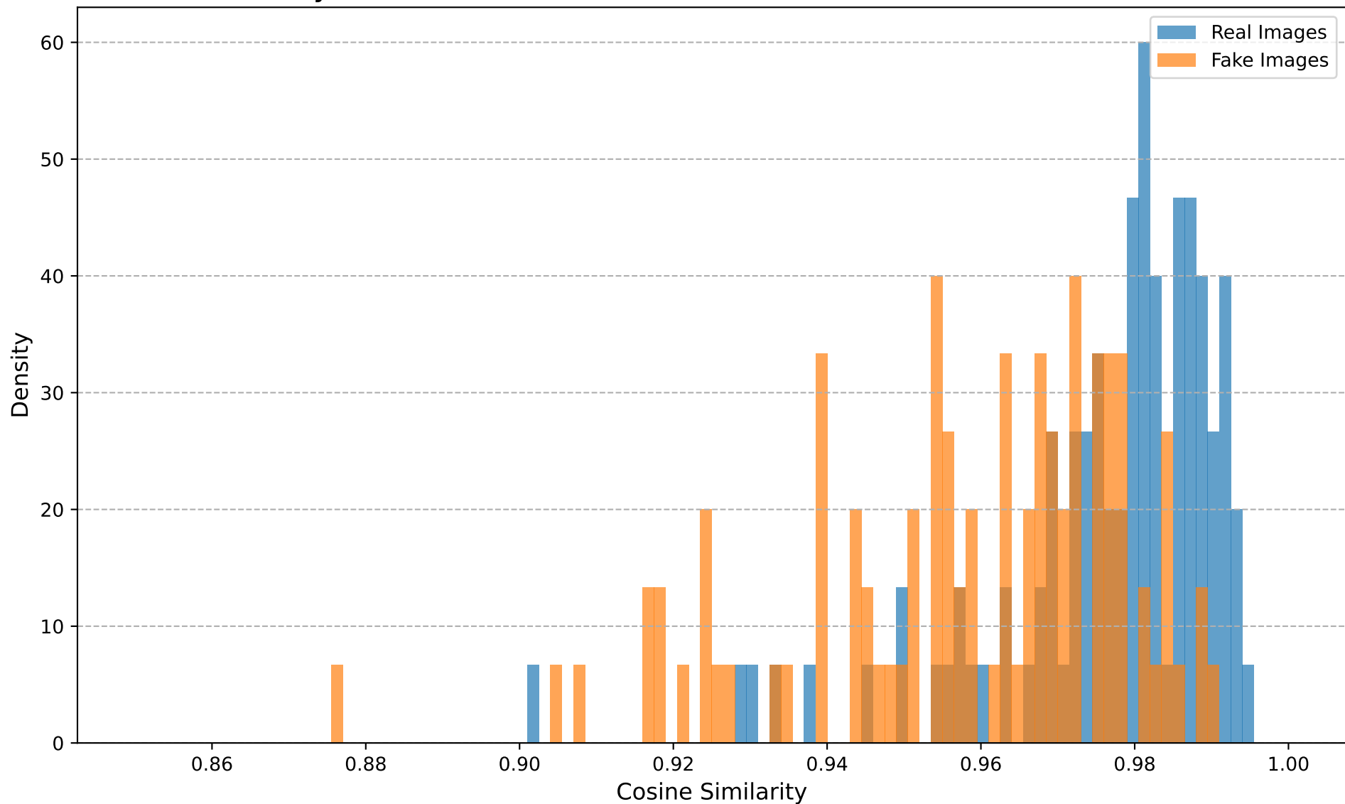
Cosine Similarity Distribution (Dataset: DALLE2, Transform: Noise, Noise STD=0.03)
