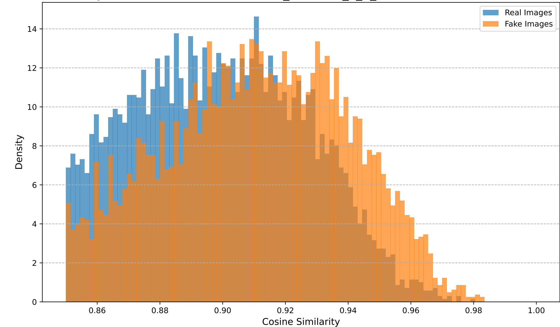
Cosine Similarity Distribution (Dataset: stable_diffusion_v_1_4, Transform: Noise, Noise STD=0.1)
