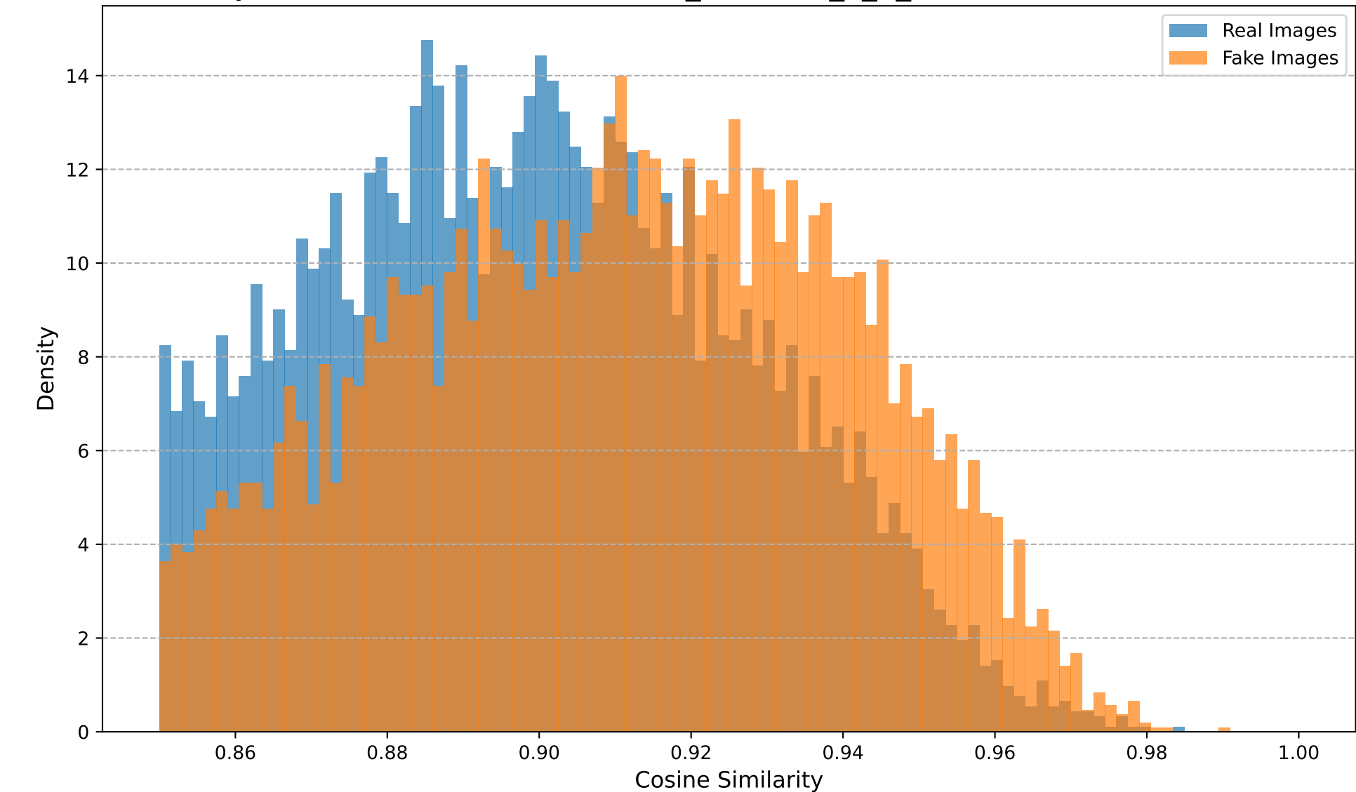
Cosine Similarity Distribution (Dataset: stable_diffusion_v_1_5, Transform: Noise, Noise STD=0.1)
