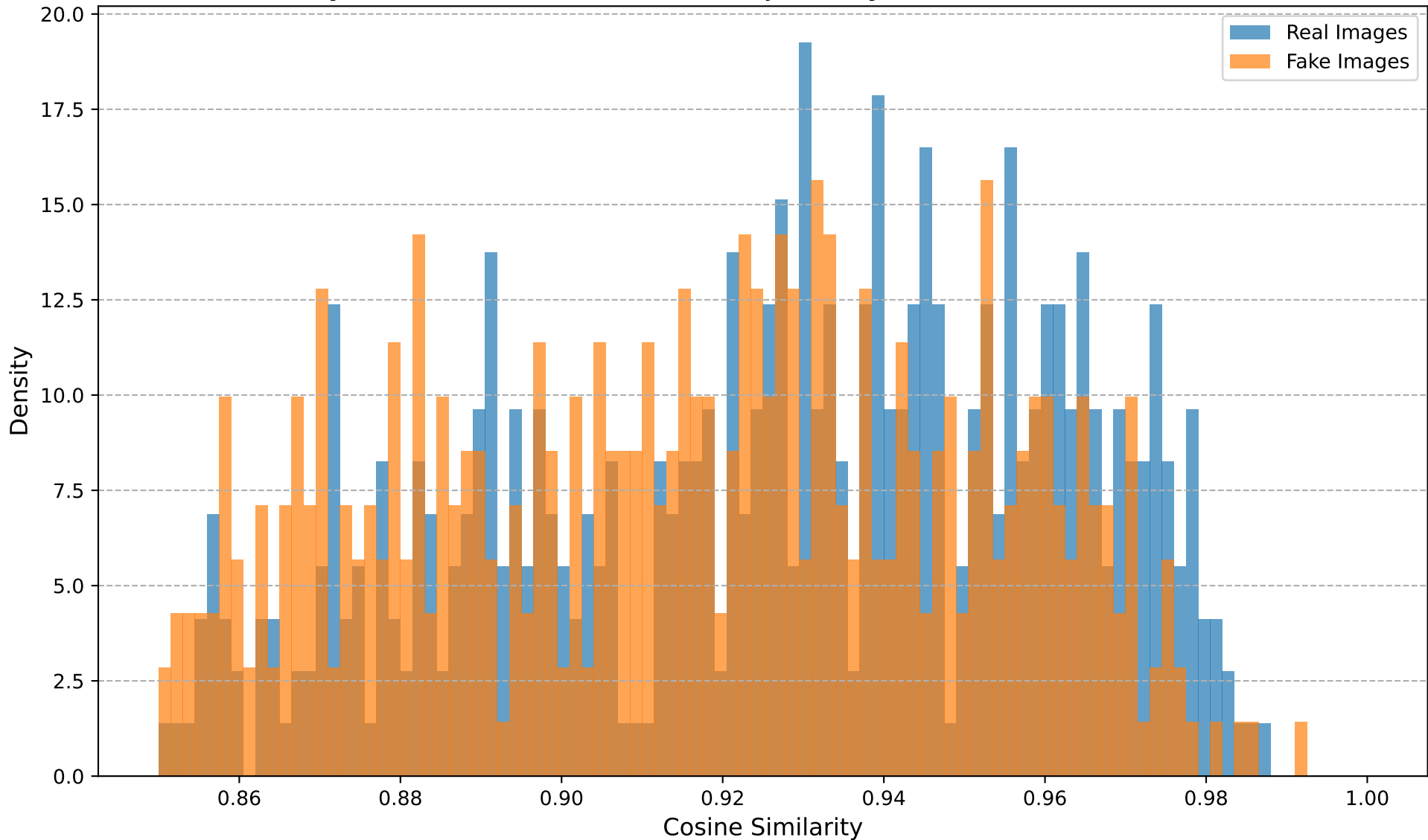
Cosine Similarity Distribution (Dataset: Midjourney, Transform: Noise, Noise STD=0.1)
