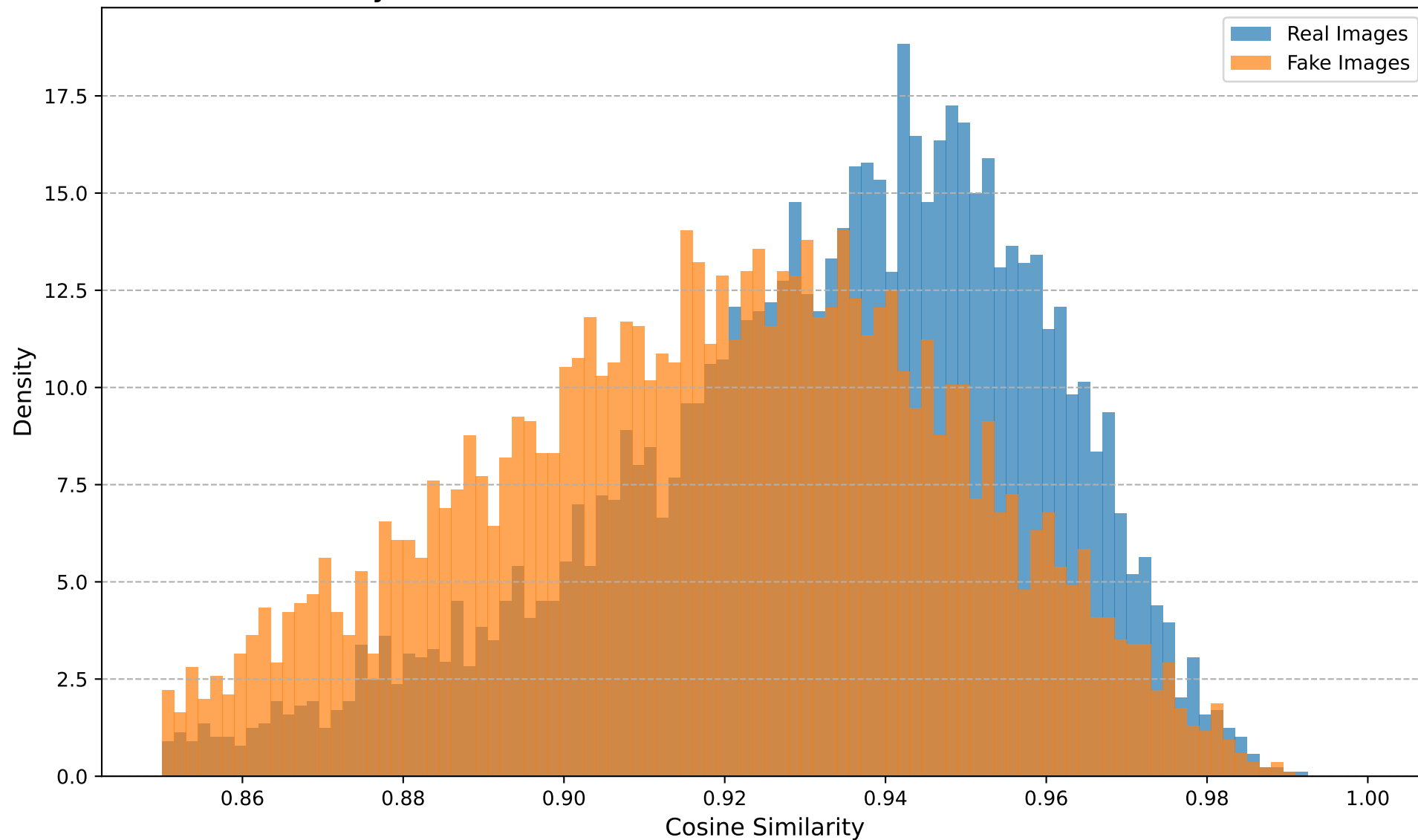
Cosine Similarity Distribution (Dataset: ADM, Transform: Noise, Noise STD=0.05)
