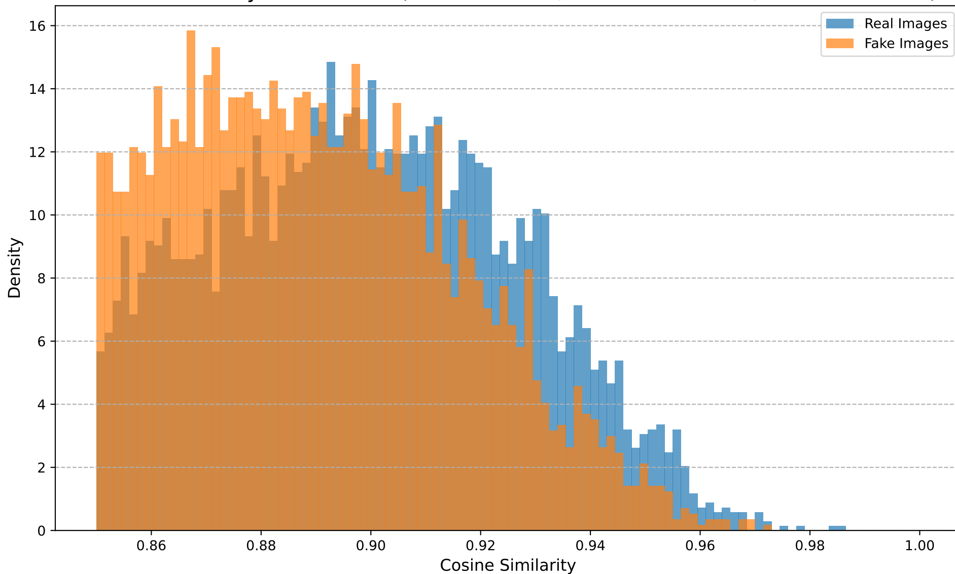
Cosine Similarity Distribution (Dataset: ADM, Transform: Noise, Noise STD=0.1)
