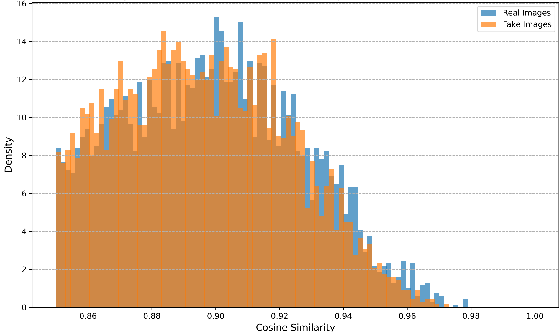
Cosine Similarity Distribution (Dataset: Midjourney, Transform: Noise, Noise STD=0.1)
