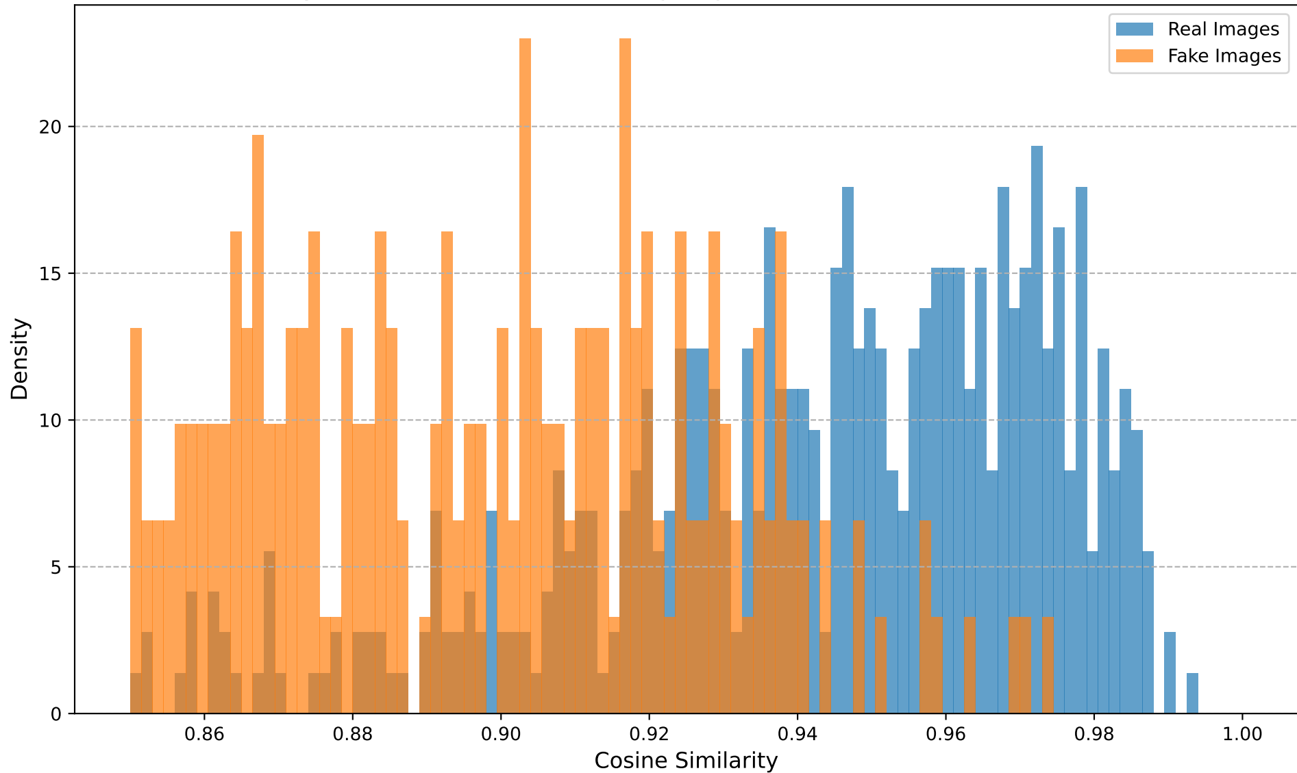
Cosine Similarity Distribution (Dataset: gaugan, Transform: Noise, Noise STD=0.05)
