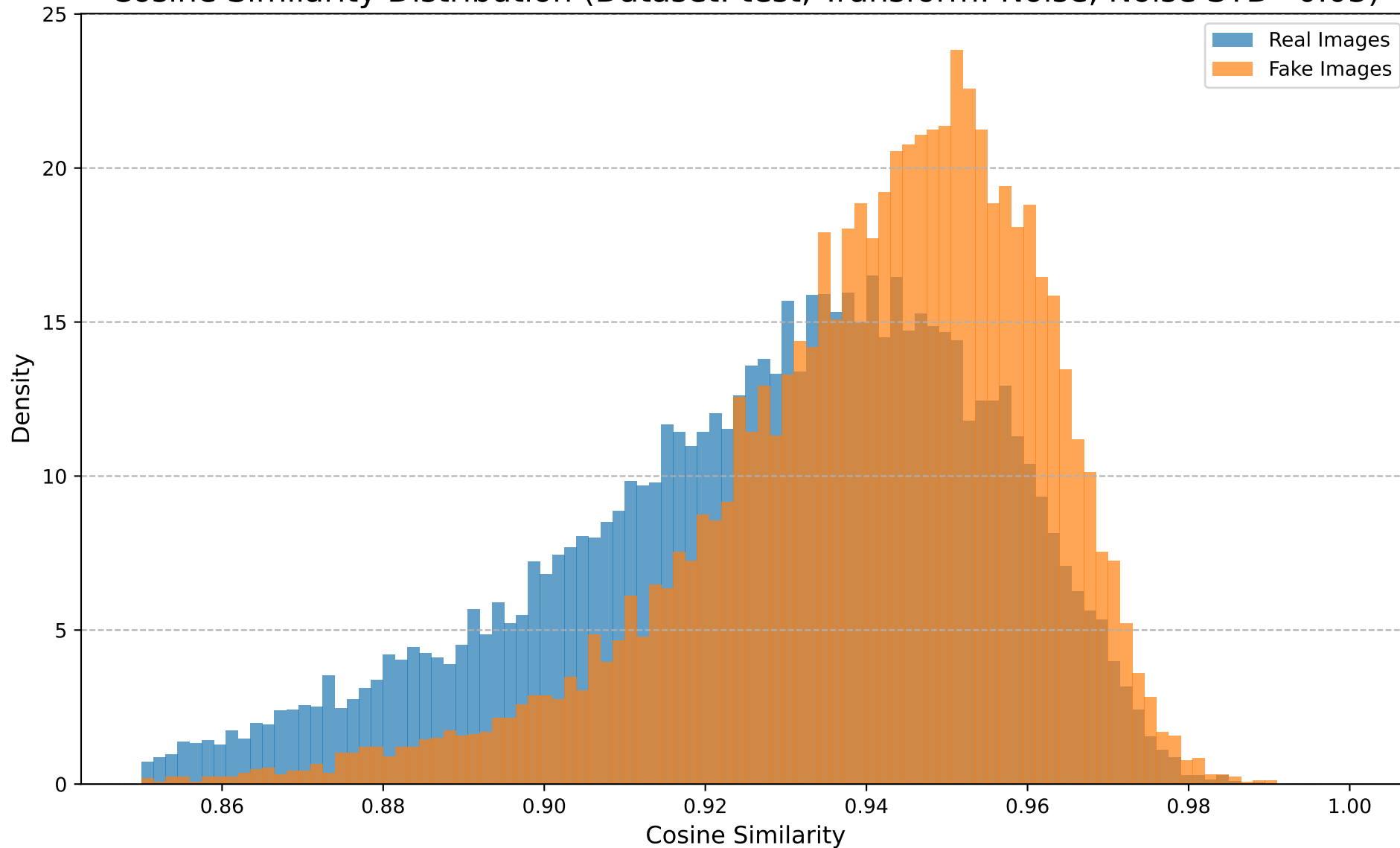
Cosine Similarity Distribution (Dataset: test, Transform: Noise, Noise STD=0.03)
