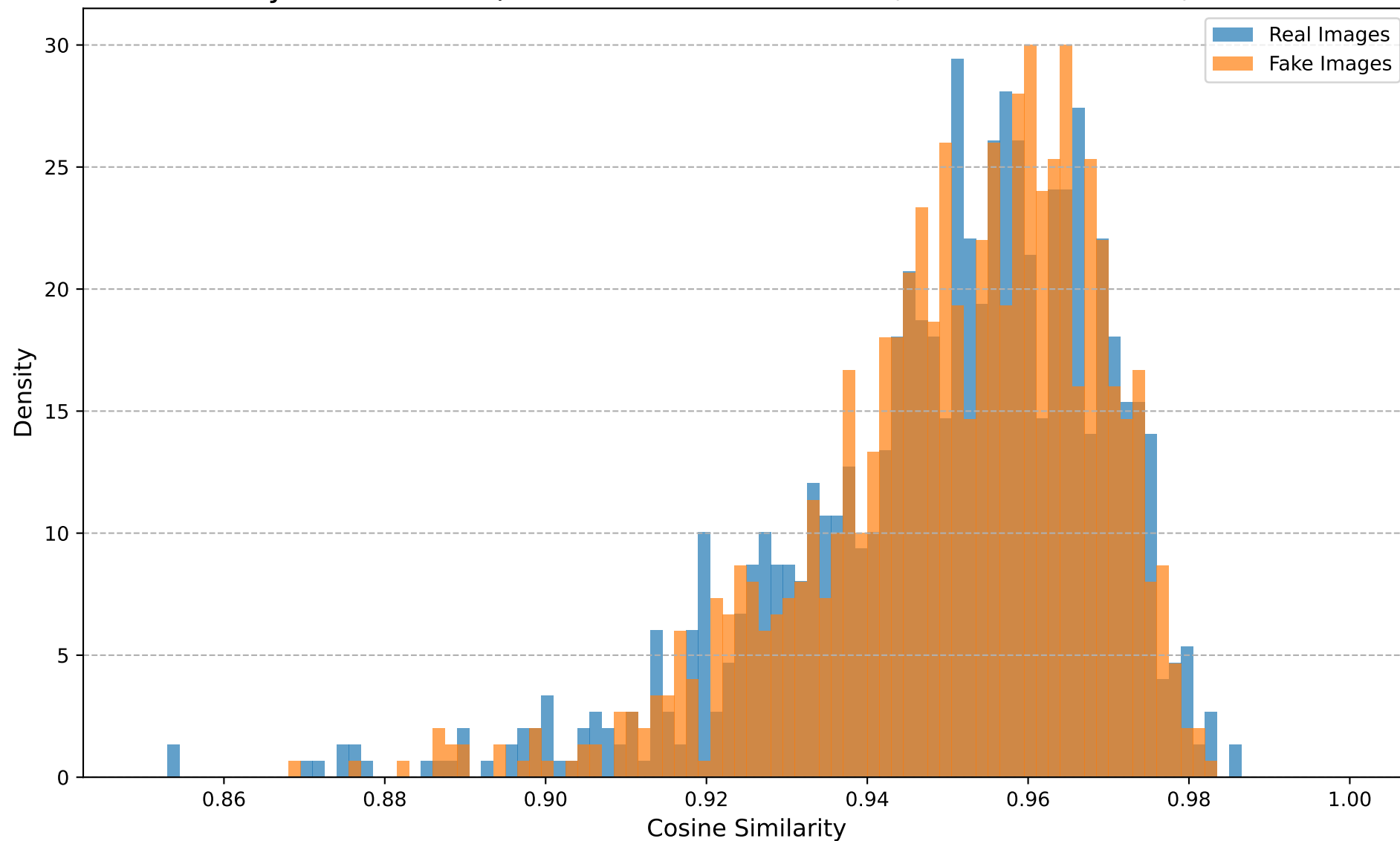
Cosine Similarity Distribution (Dataset: whichfaceisreal, Transform: Noise, Noise STD=0.03)
