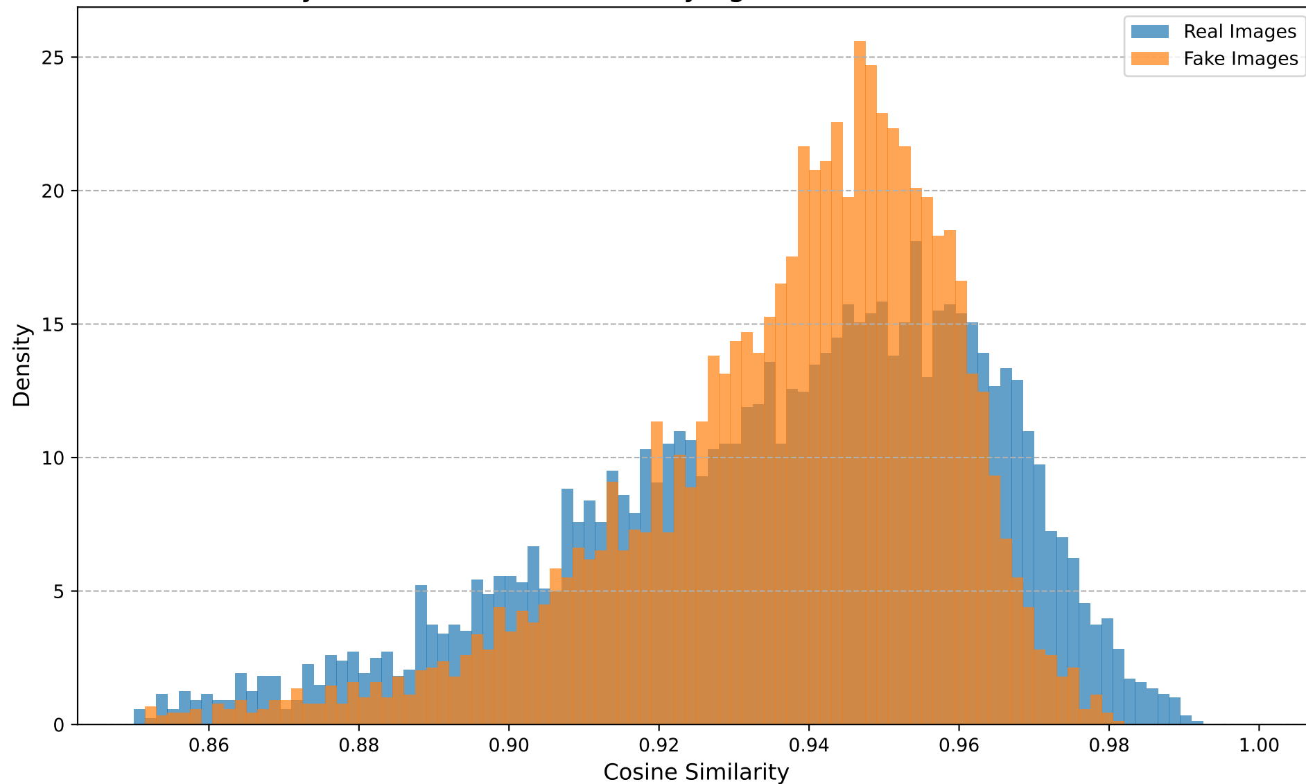
Cosine Similarity Distribution (Dataset: stylegan, Transform: Noise, Noise STD=0.03)
