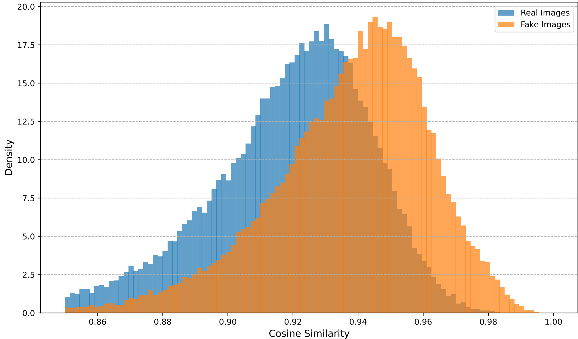
Cosine Similarity Distribution (Transform: Blur, Blur Sigma=1.0)
