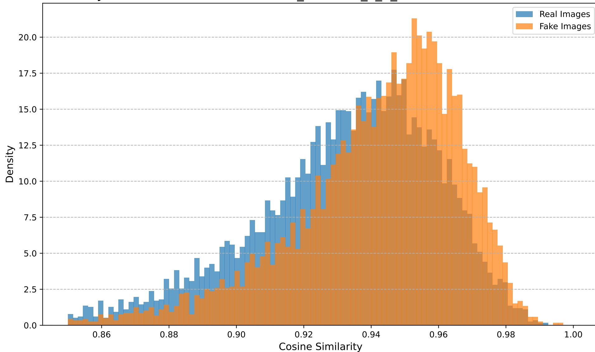
Cosine Similarity Distribution (Dataset: stable_diffusion_v_1_5, Transform: Noise, Noise STD=0.05)
