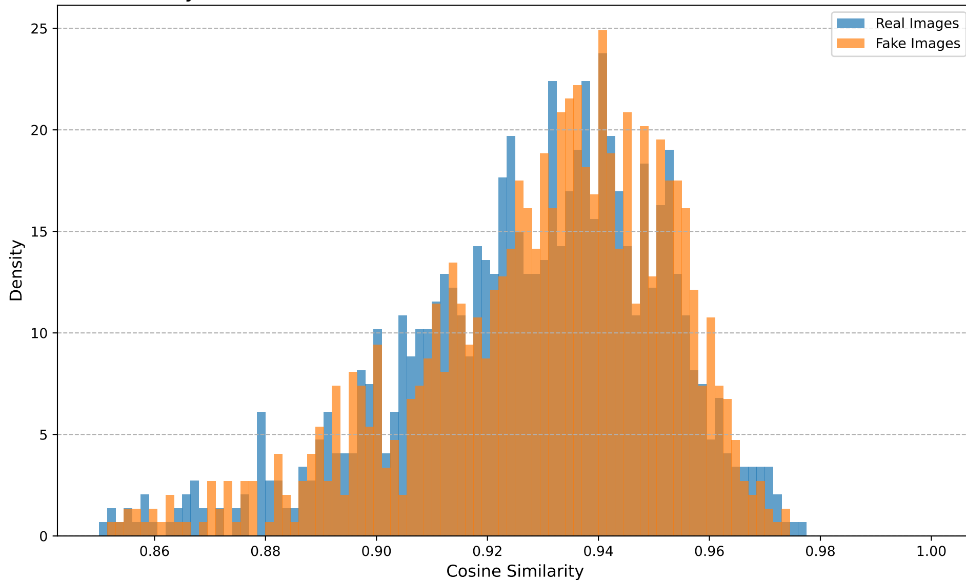
Cosine Similarity Distribution (Dataset: whichfaceisreal, Transform: Noise, Noise STD=0.05)
