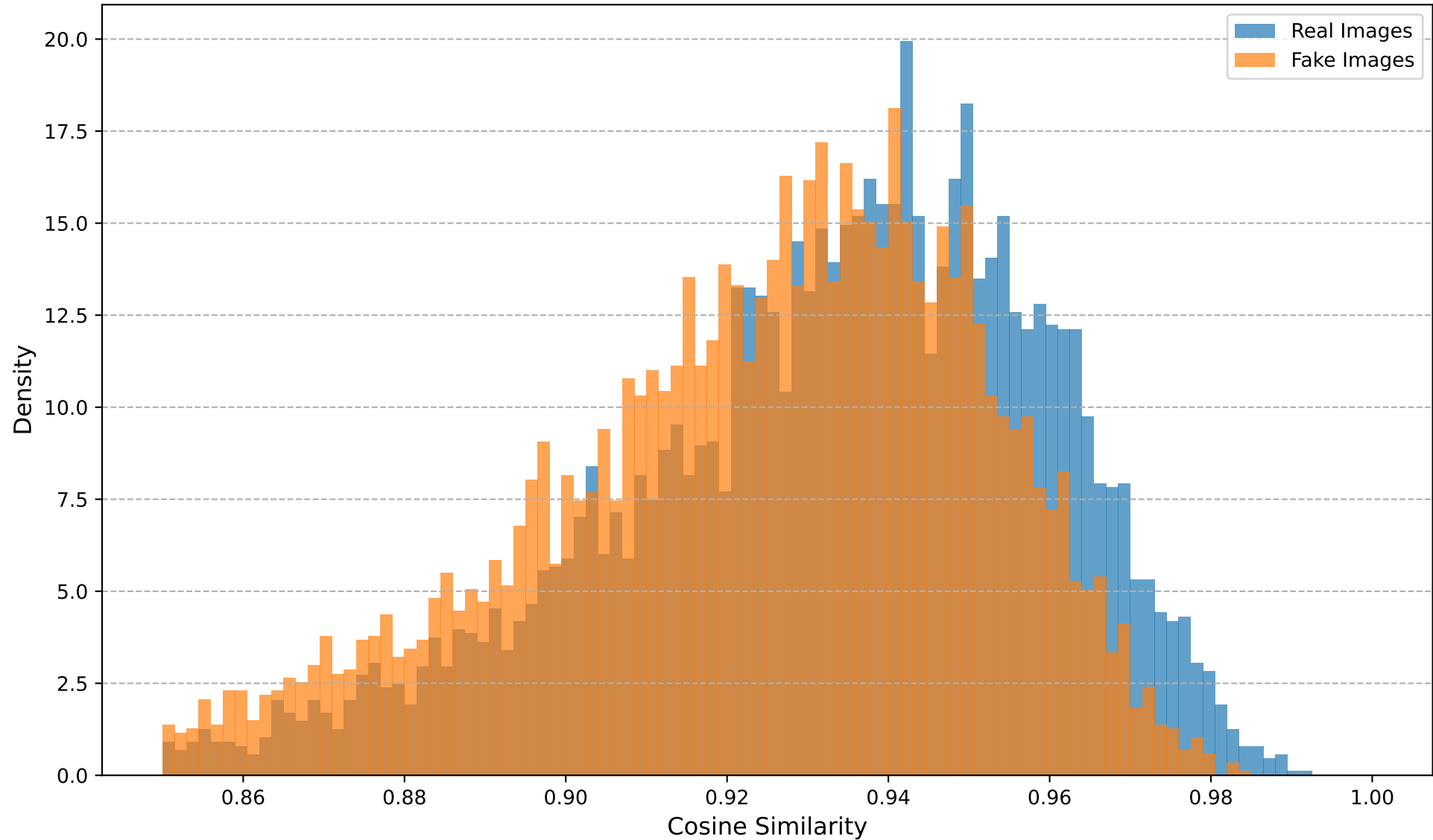
Cosine Similarity Distribution (Dataset: Midjourney, Transform: Noise, Noise STD=0.05)
