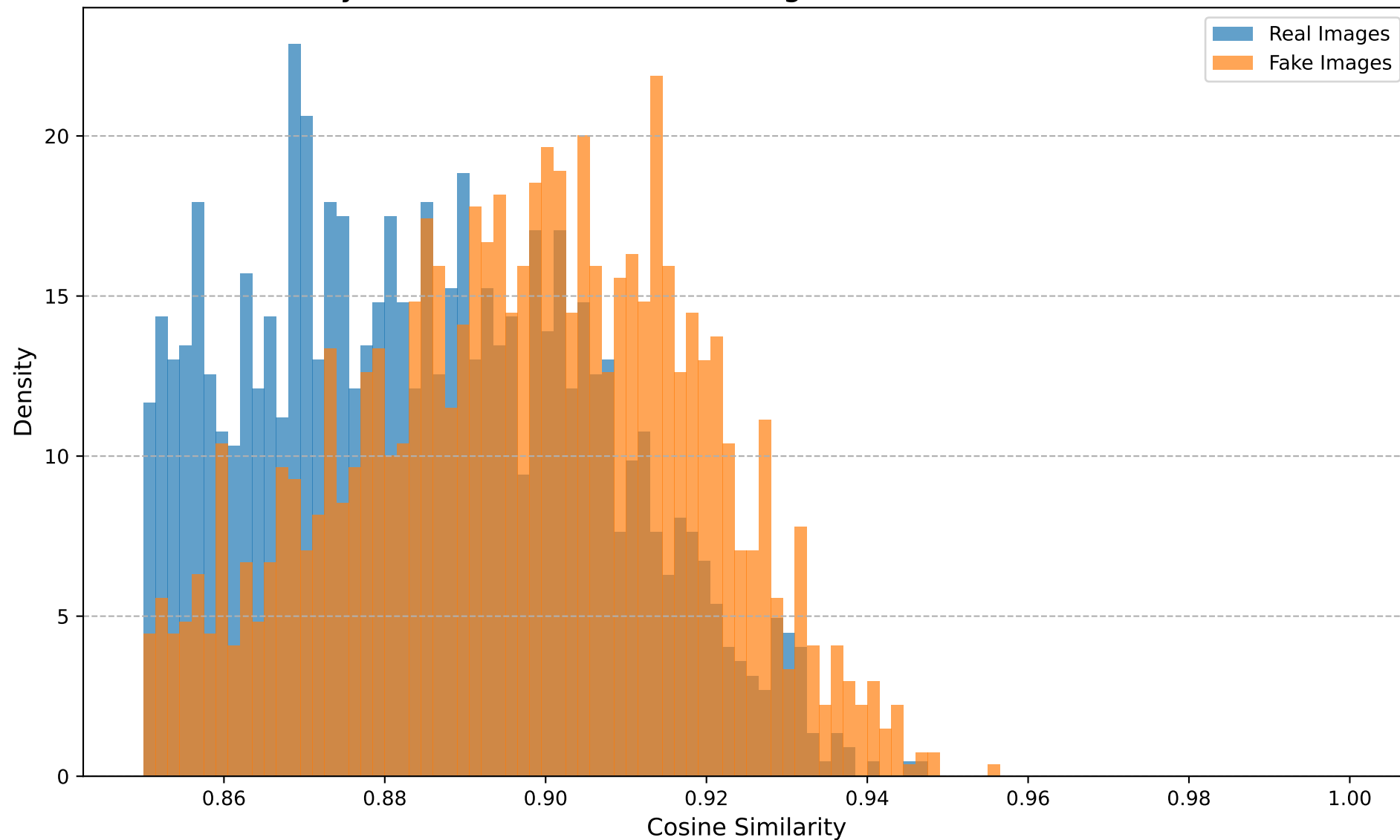
Cosine Similarity Distribution (Dataset: stargan, Transform: Noise, Noise STD=0.1)
