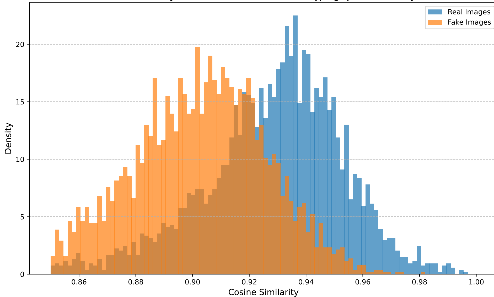
Cosine Similarity Distribution (Transform: jpeg, JPEG Quality=50)
