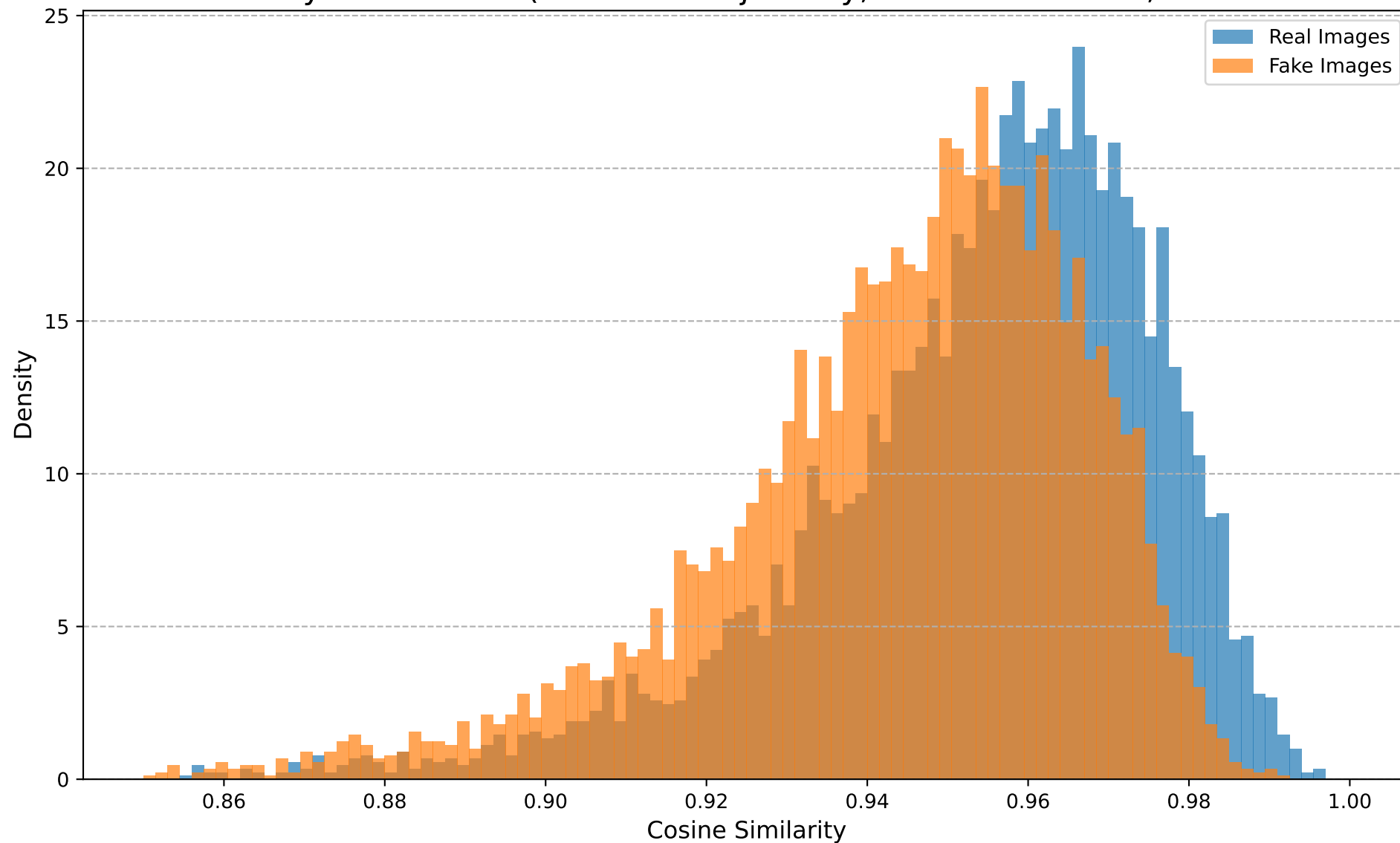
Cosine Similarity Distribution (Dataset: Midjourney, Transform: Noise, Noise STD=0.03)
