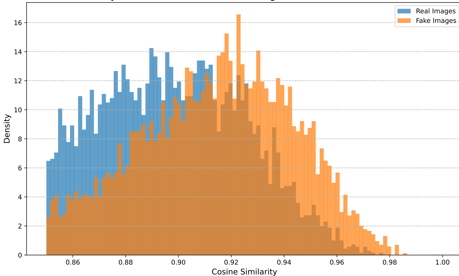
Cosine Similarity Distribution (Dataset: wukong, Transform: Noise, Noise STD=0.1)
