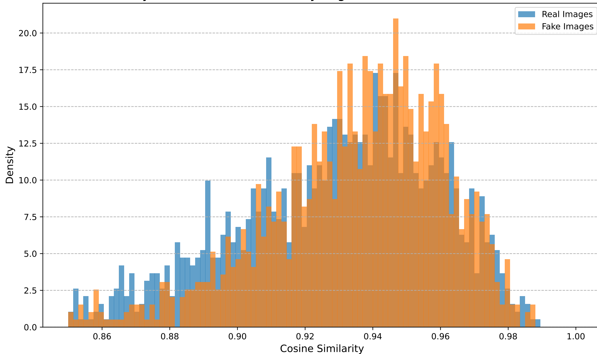
Cosine Similarity Distribution (Dataset: cyclegan, Transform: Noise, Noise STD=0.05)
