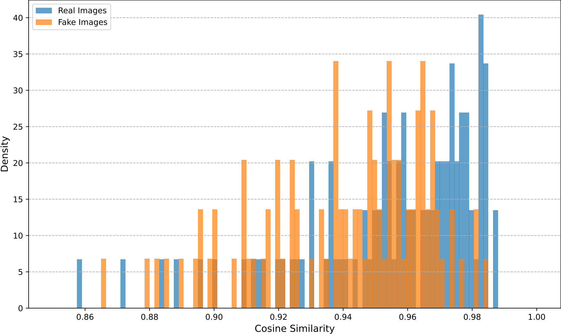
Cosine Similarity Distribution (Dataset: DALLE2, Transform: Noise, Noise STD=0.05)
