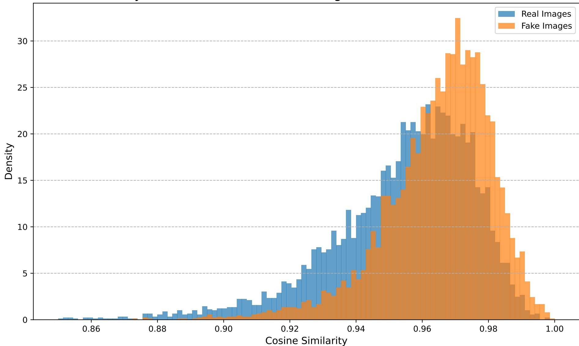
Cosine Similarity Distribution (Dataset: wukong, Transform: Noise, Noise STD=0.03)
