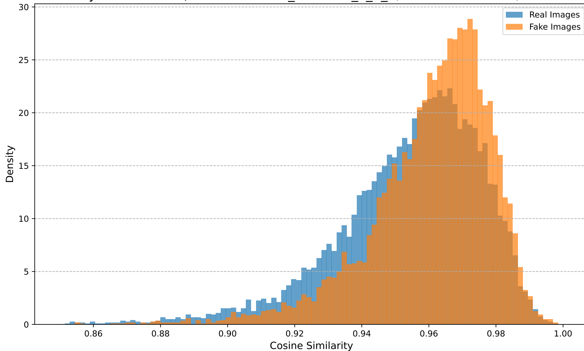
Cosine Similarity Distribution (Dataset: stable_diffusion_v_1_5, Transform: Noise, Noise STD=0.03)
