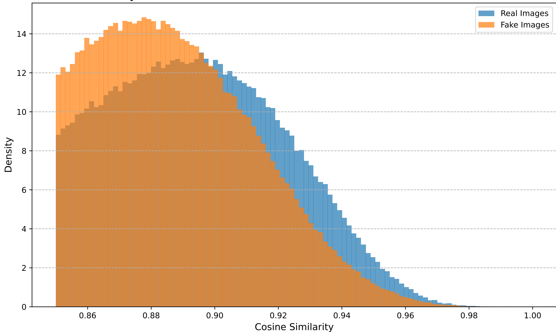
Cosine Similarity Distribution (Dataset: Datasets, Transform: Noise, Noise STD=0.1)
