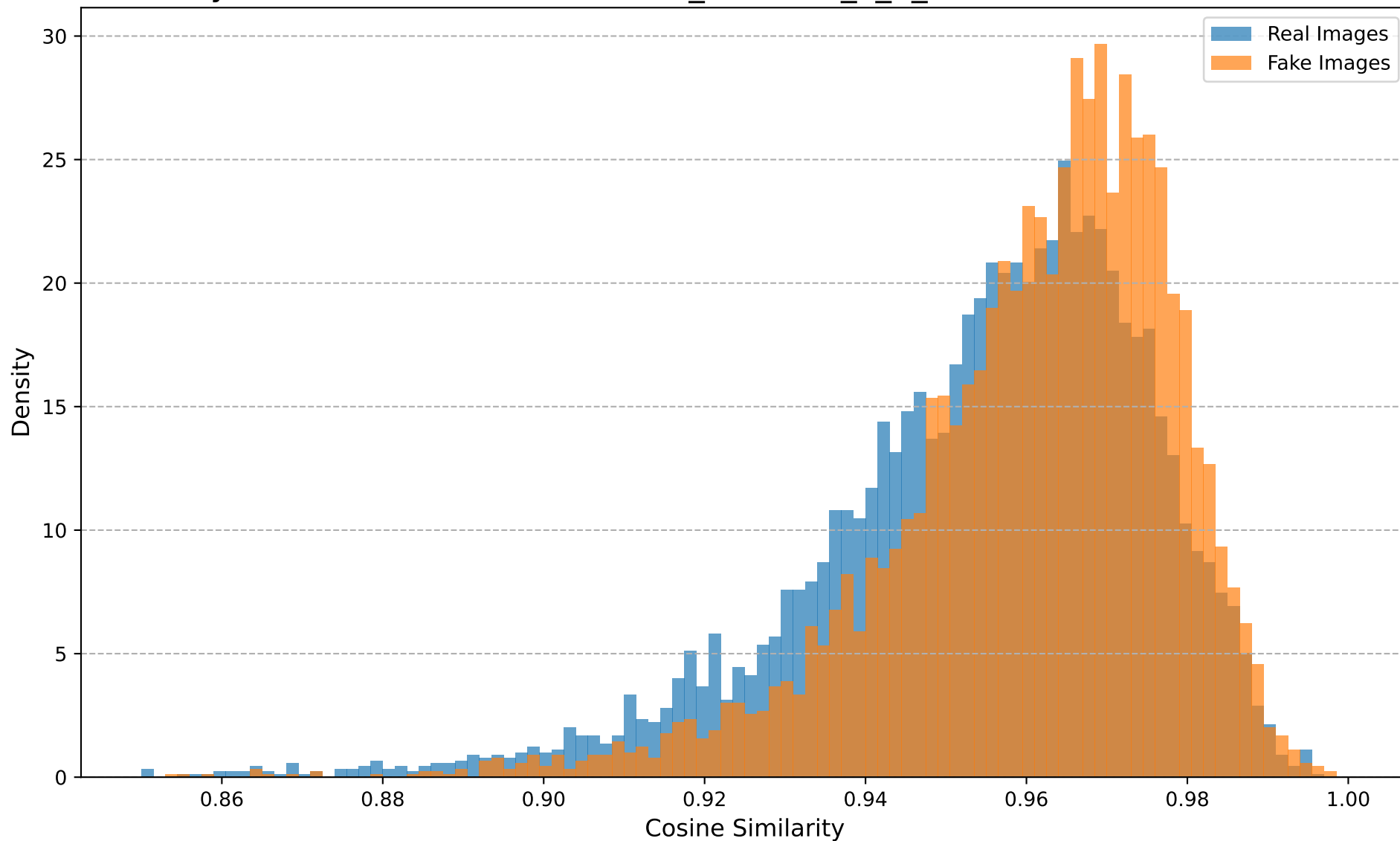
Cosine Similarity Distribution (Dataset: stable_diffusion_v_1_4, Transform: Noise, Noise STD=0.03)
