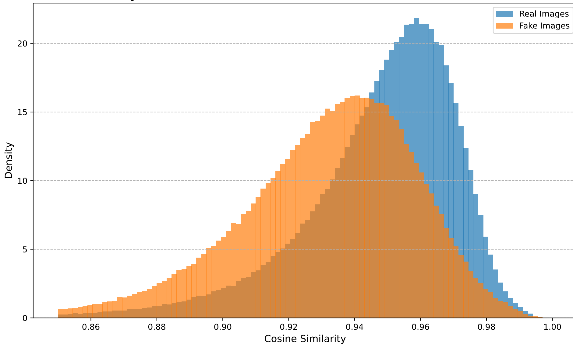
Cosine Similarity Distribution (Dataset: Datasets, Transform: Noise, Noise STD=0.03)
