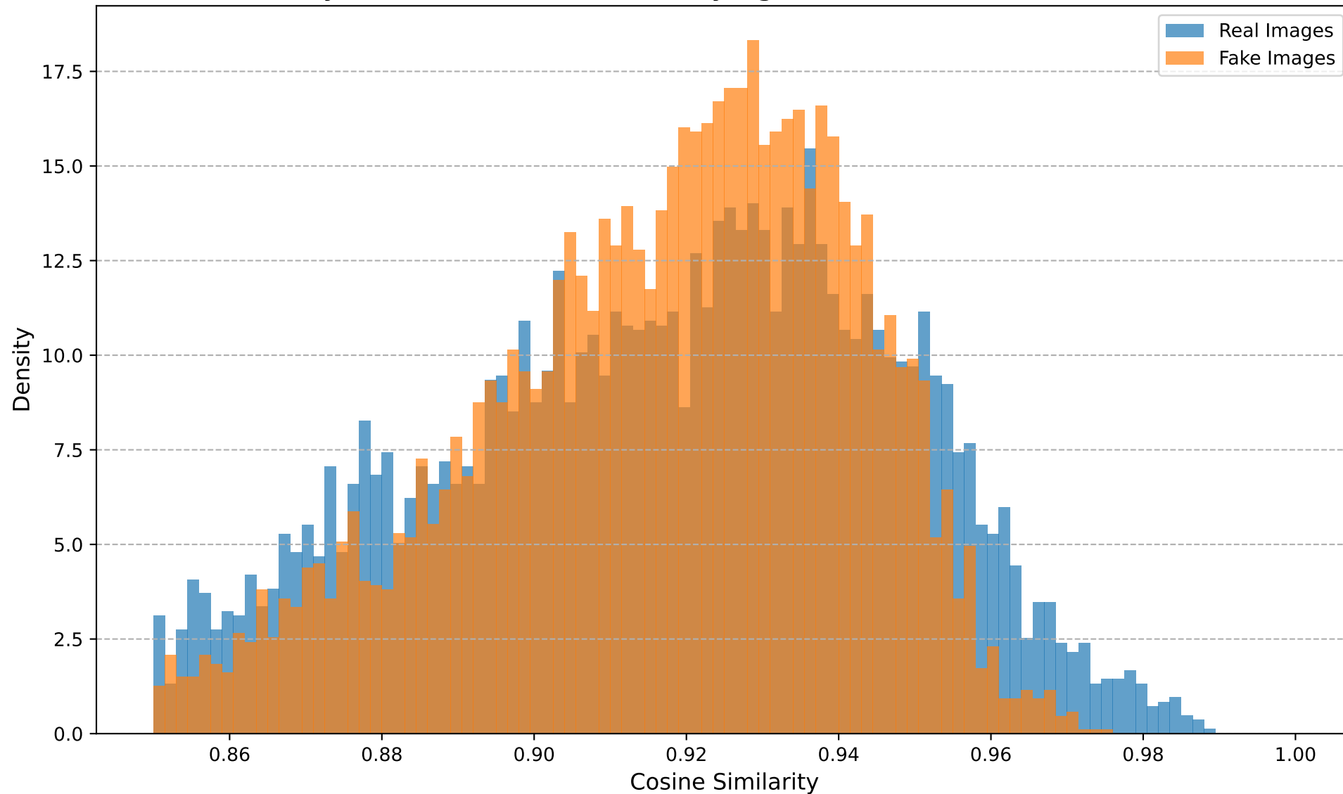
Cosine Similarity Distribution (Dataset: stylegan, Transform: Noise, Noise STD=0.05)
