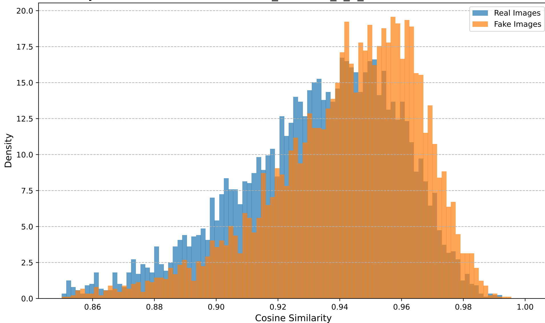
Cosine Similarity Distribution (Dataset: stable_diffusion_v_1_4, Transform: Noise, Noise STD=0.05)
