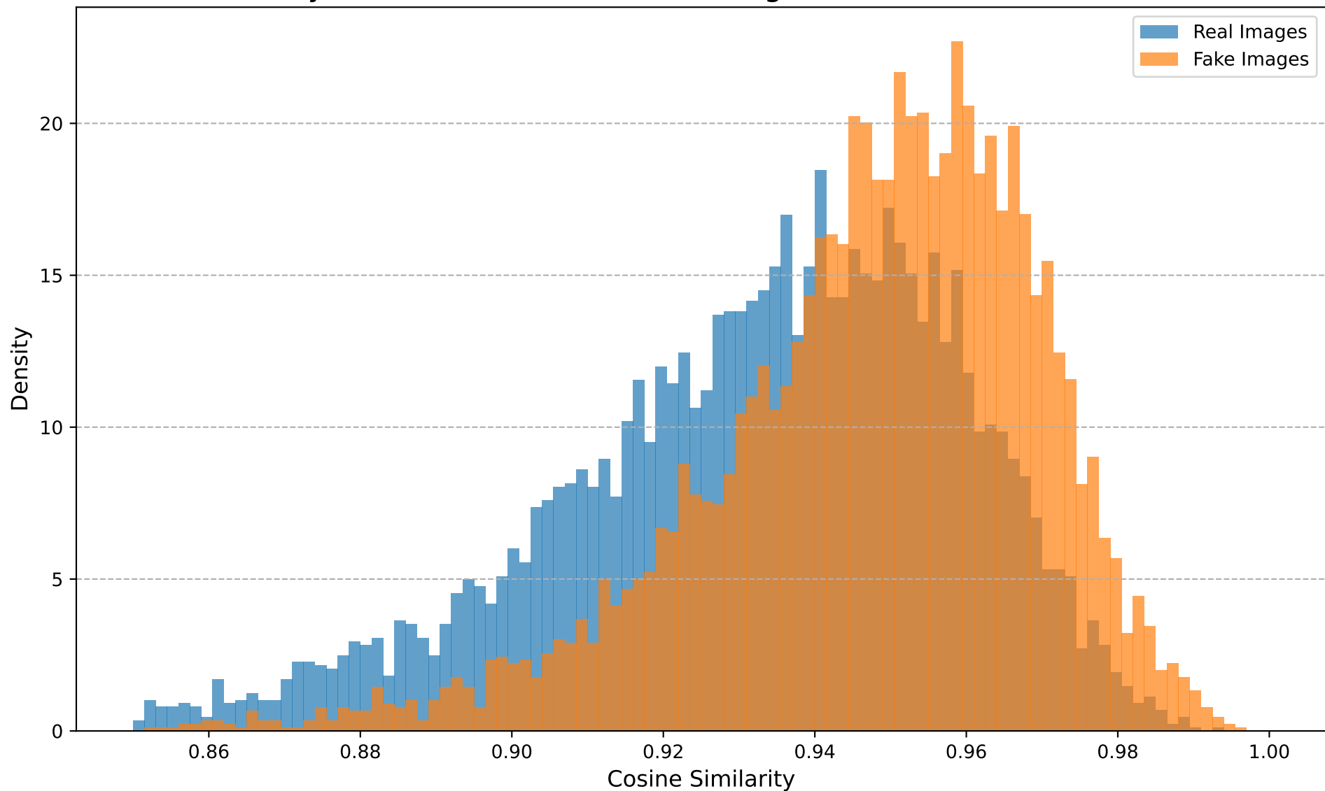
Cosine Similarity Distribution (Dataset: wukong, Transform: Noise, Noise STD=0.05)
