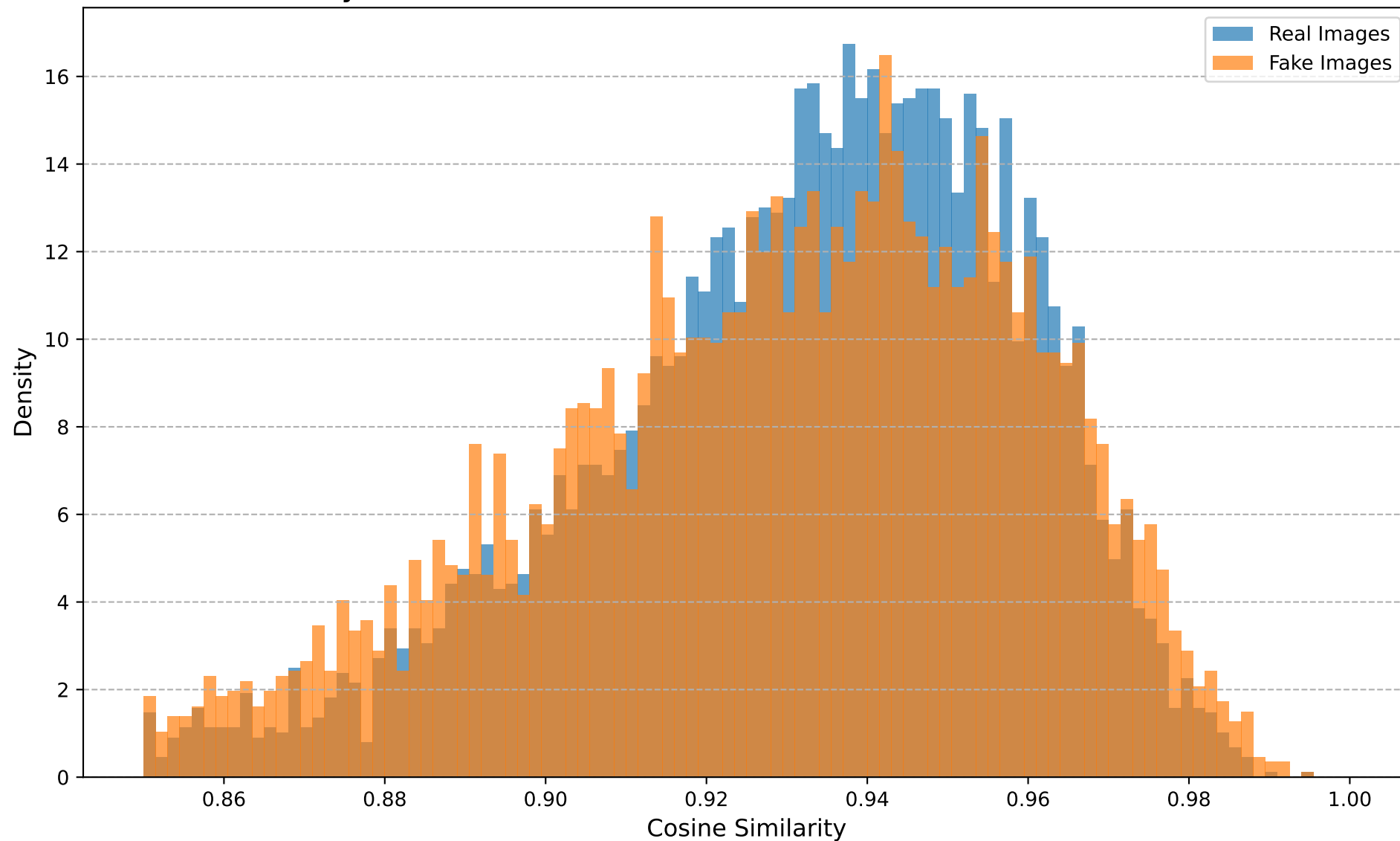
Cosine Similarity Distribution (Dataset: VQDM, Transform: Noise, Noise STD=0.05)
