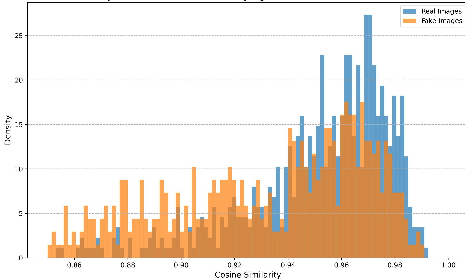
Cosine Similarity Distribution (Dataset: stylegan, Transform: Noise, Noise STD=0.05)
