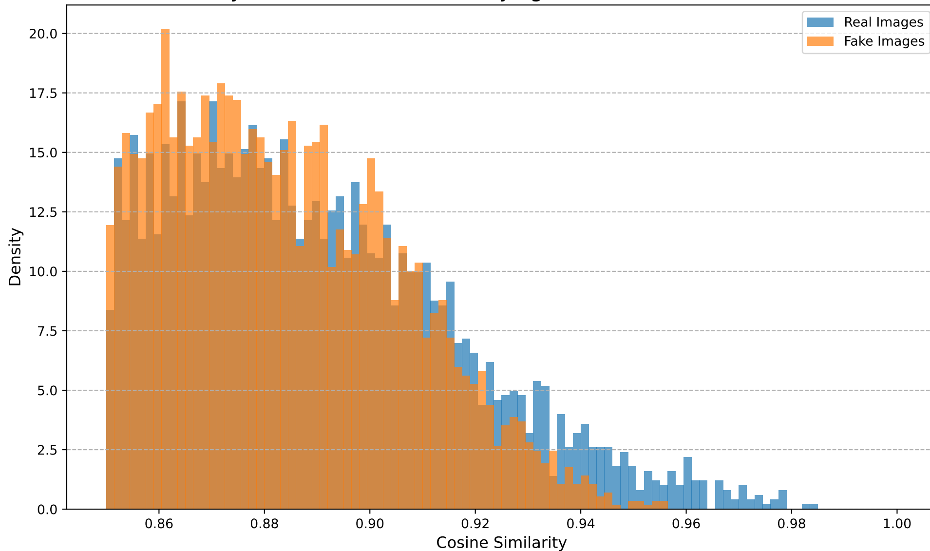
Cosine Similarity Distribution (Dataset: stylegan, Transform: Noise, Noise STD=0.1)
