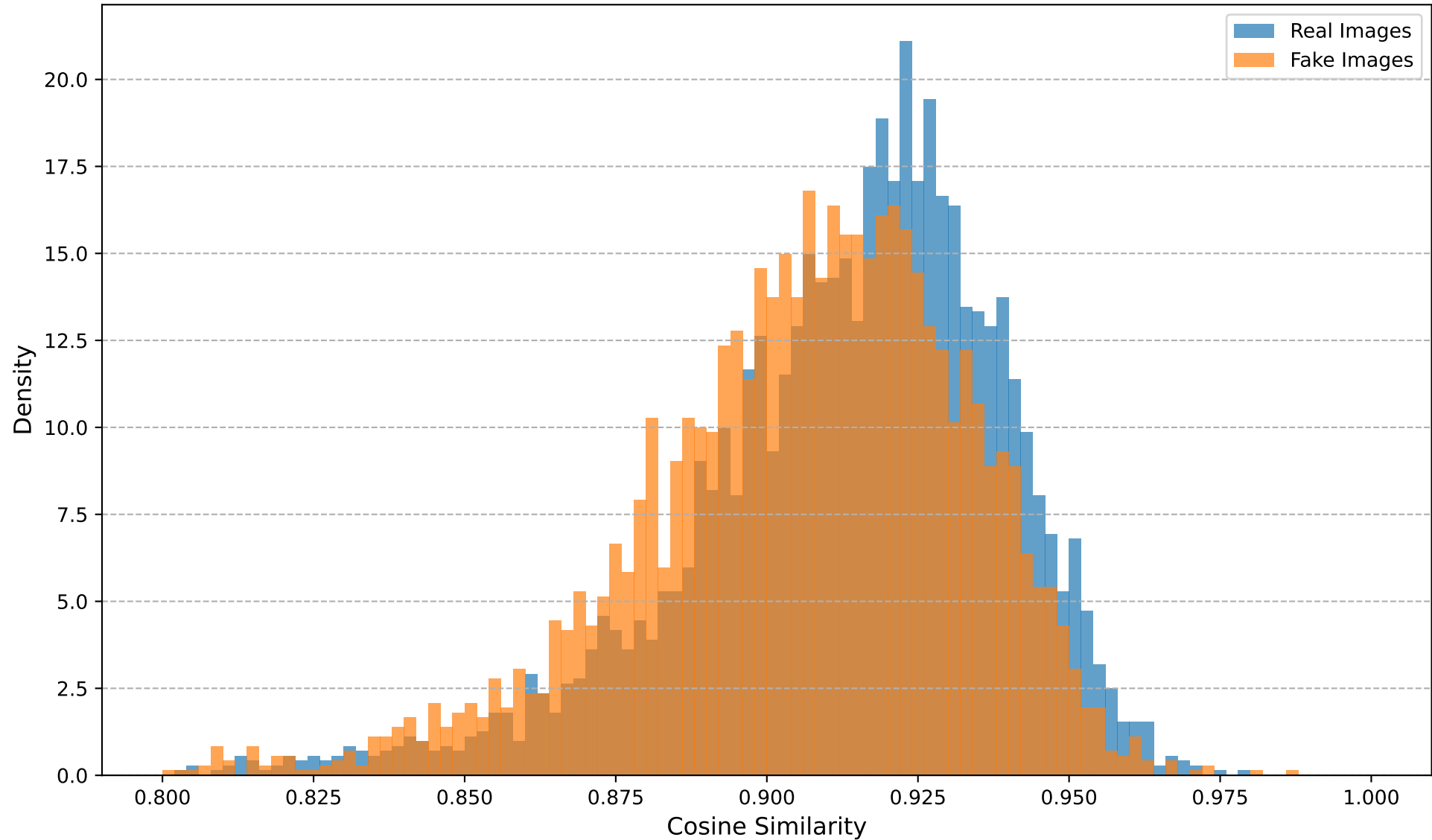
Cosine Similarity Distribution (Transform: Blur, Blur Sigma=1.2)
