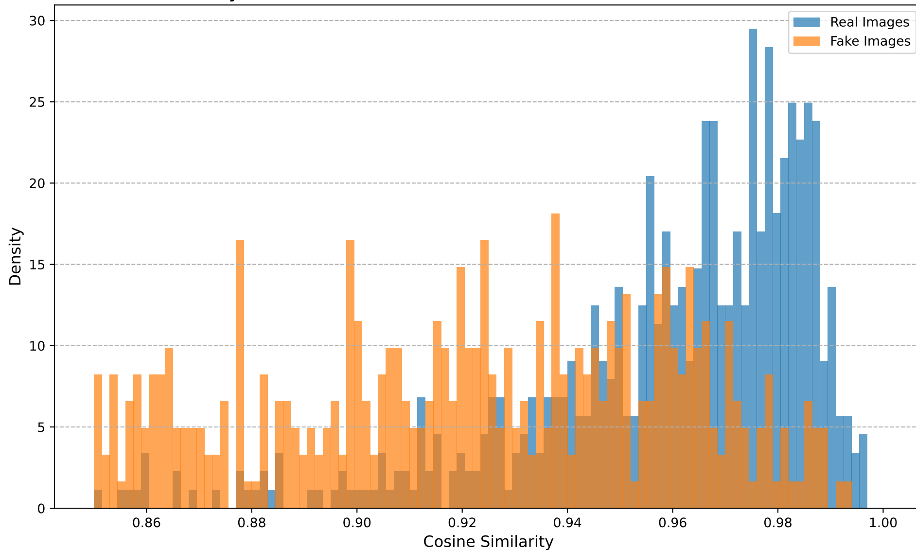
Cosine Similarity Distribution (Dataset: Glide, Transform: Noise, Noise STD=0.05)
