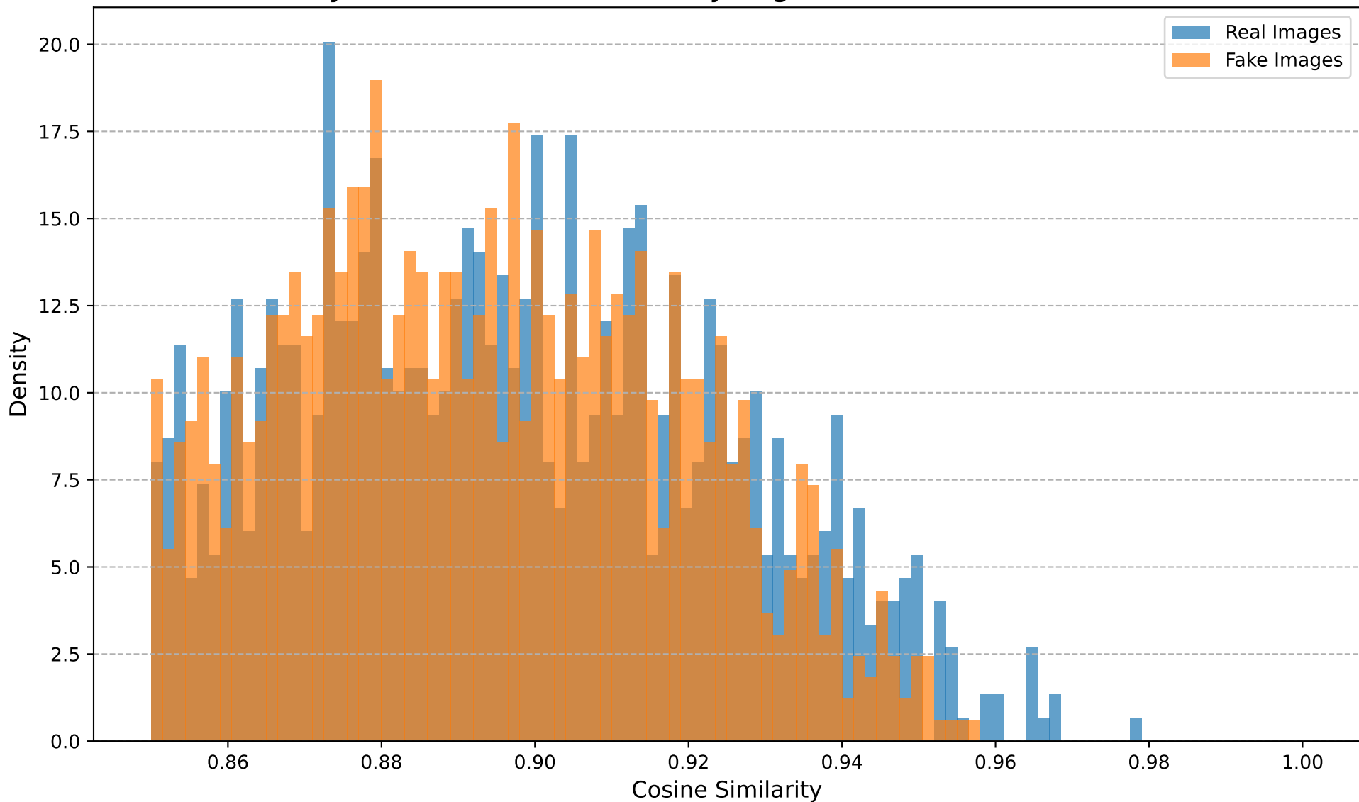
Cosine Similarity Distribution (Dataset: cyclegan, Transform: Noise, Noise STD=0.1)
