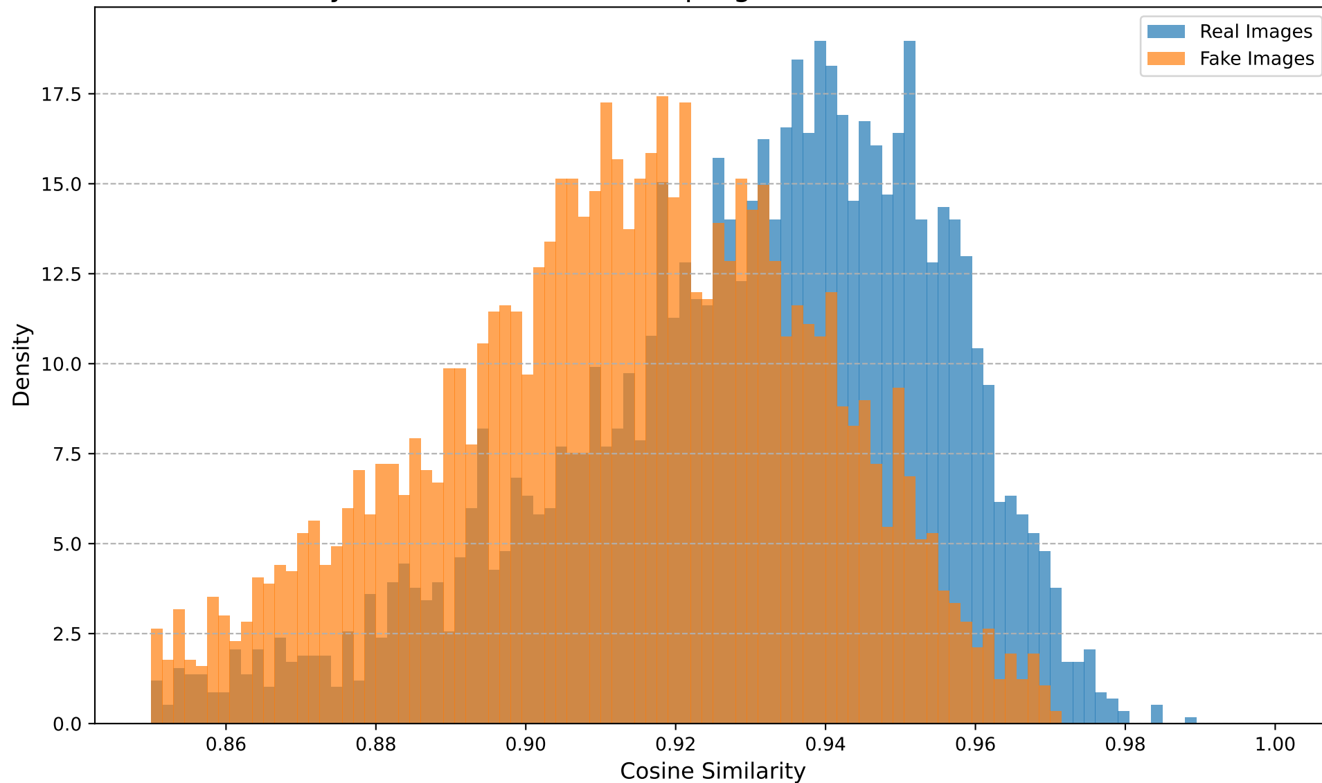
Cosine Similarity Distribution (Dataset: progan, Transform: Noise, Noise STD=0.05)
