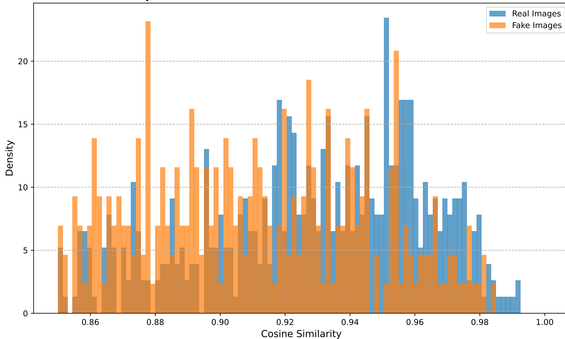
Cosine Similarity Distribution (Dataset: Glide, Transform: Noise, Noise STD=0.1)
