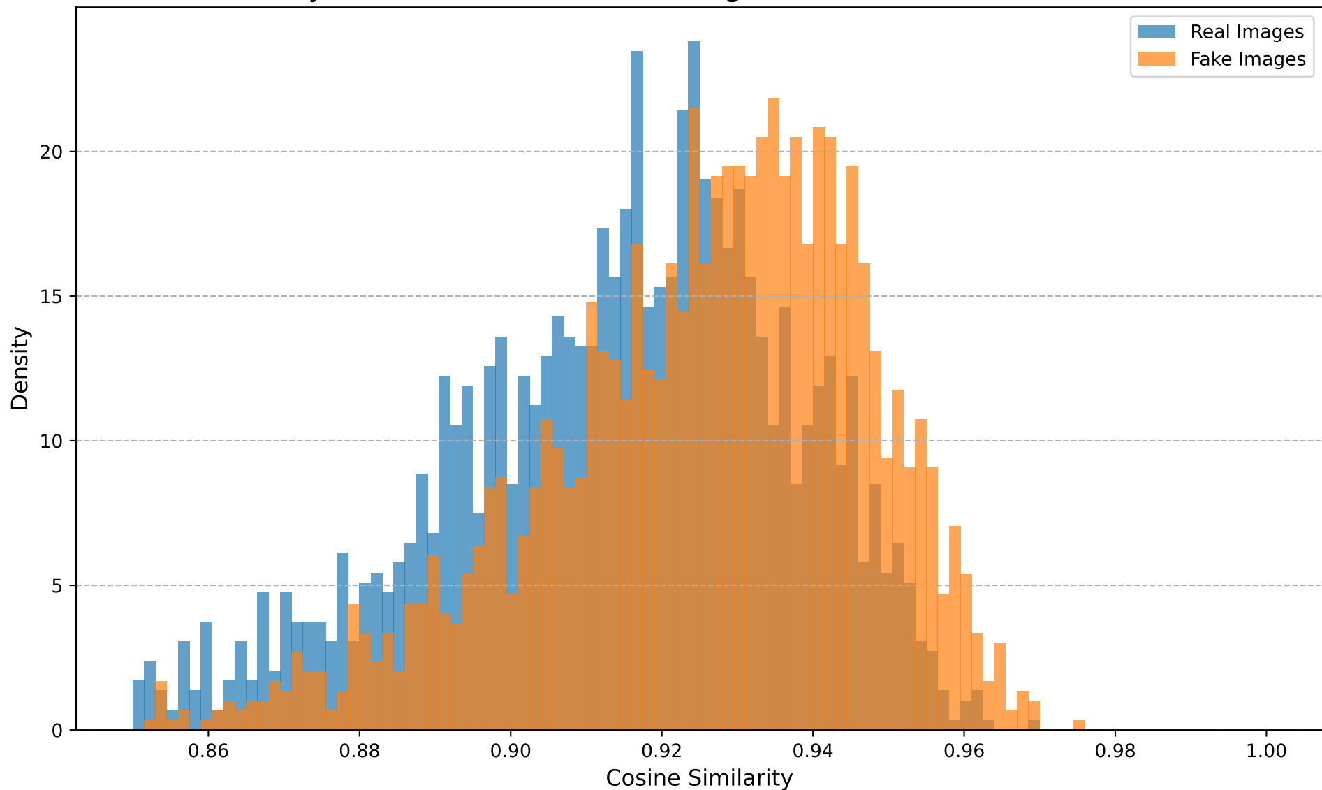
Cosine Similarity Distribution (Dataset: stargan, Transform: Noise, Noise STD=0.05)
