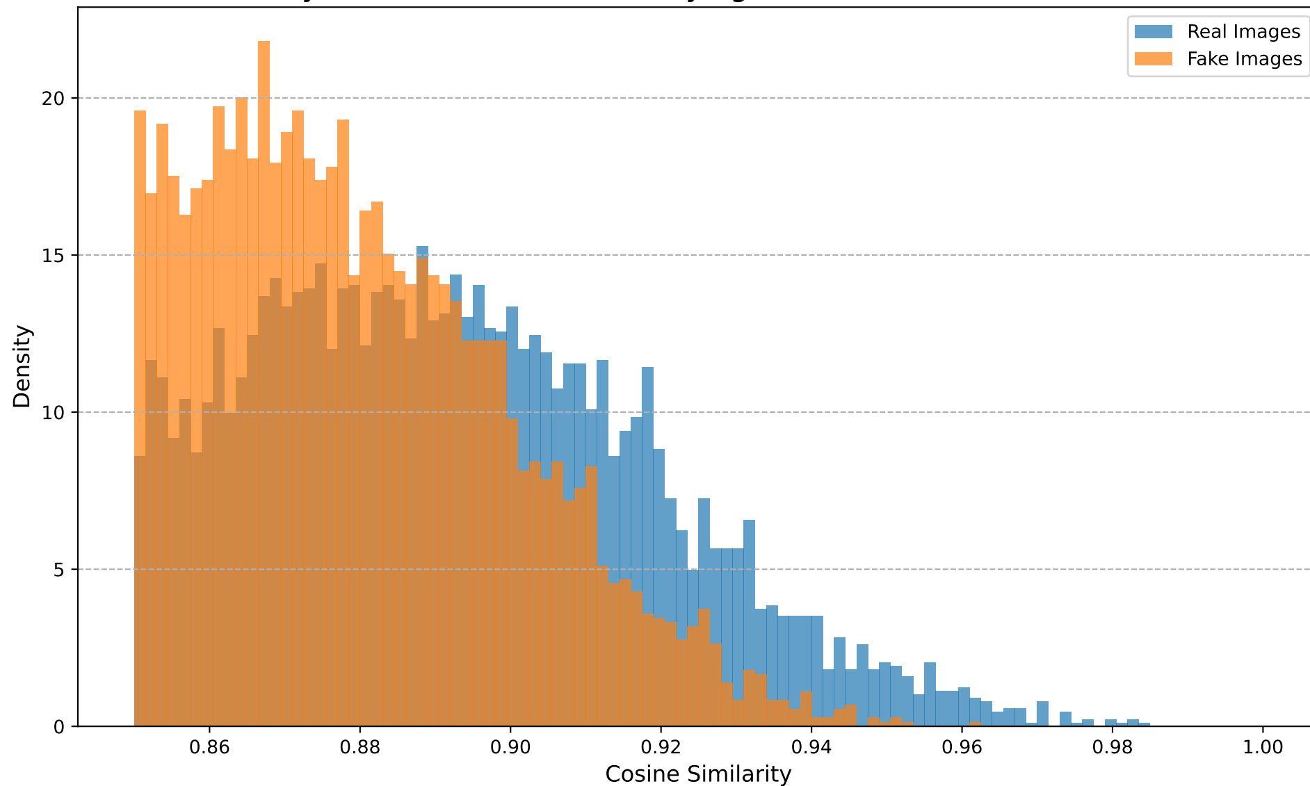
Cosine Similarity Distribution (Dataset: stylegan2, Transform: Noise, Noise STD=0.1)
