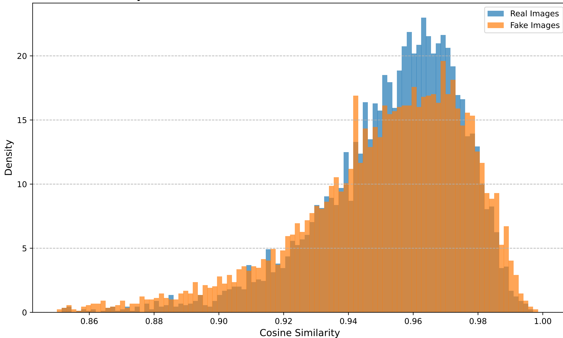
Cosine Similarity Distribution (Dataset: VQDM, Transform: Noise, Noise STD=0.03)
