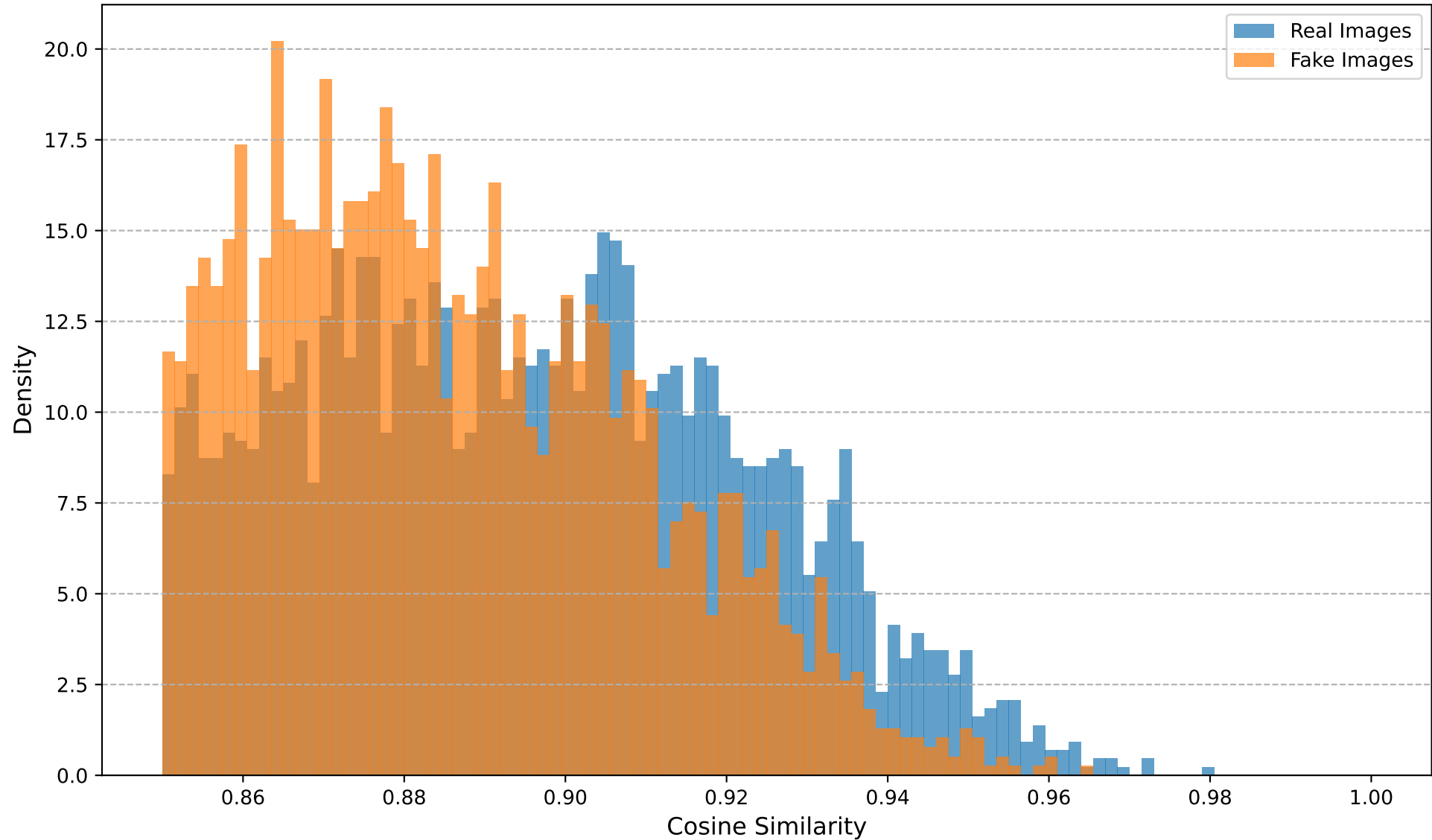
Cosine Similarity Distribution (Dataset: progan, Transform: Noise, Noise STD=0.1)
