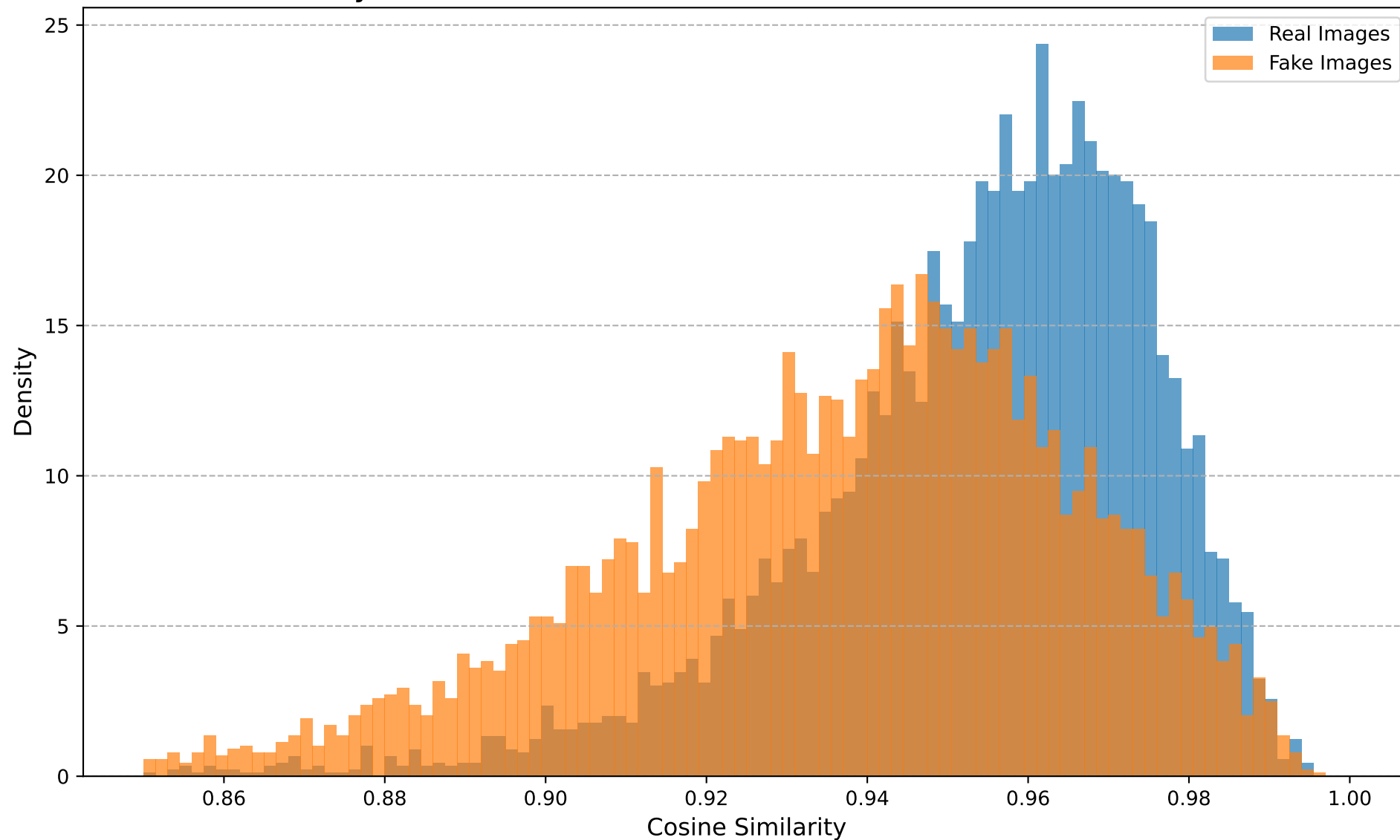
Cosine Similarity Distribution (Dataset: ADM, Transform: Noise, Noise STD=0.03)
