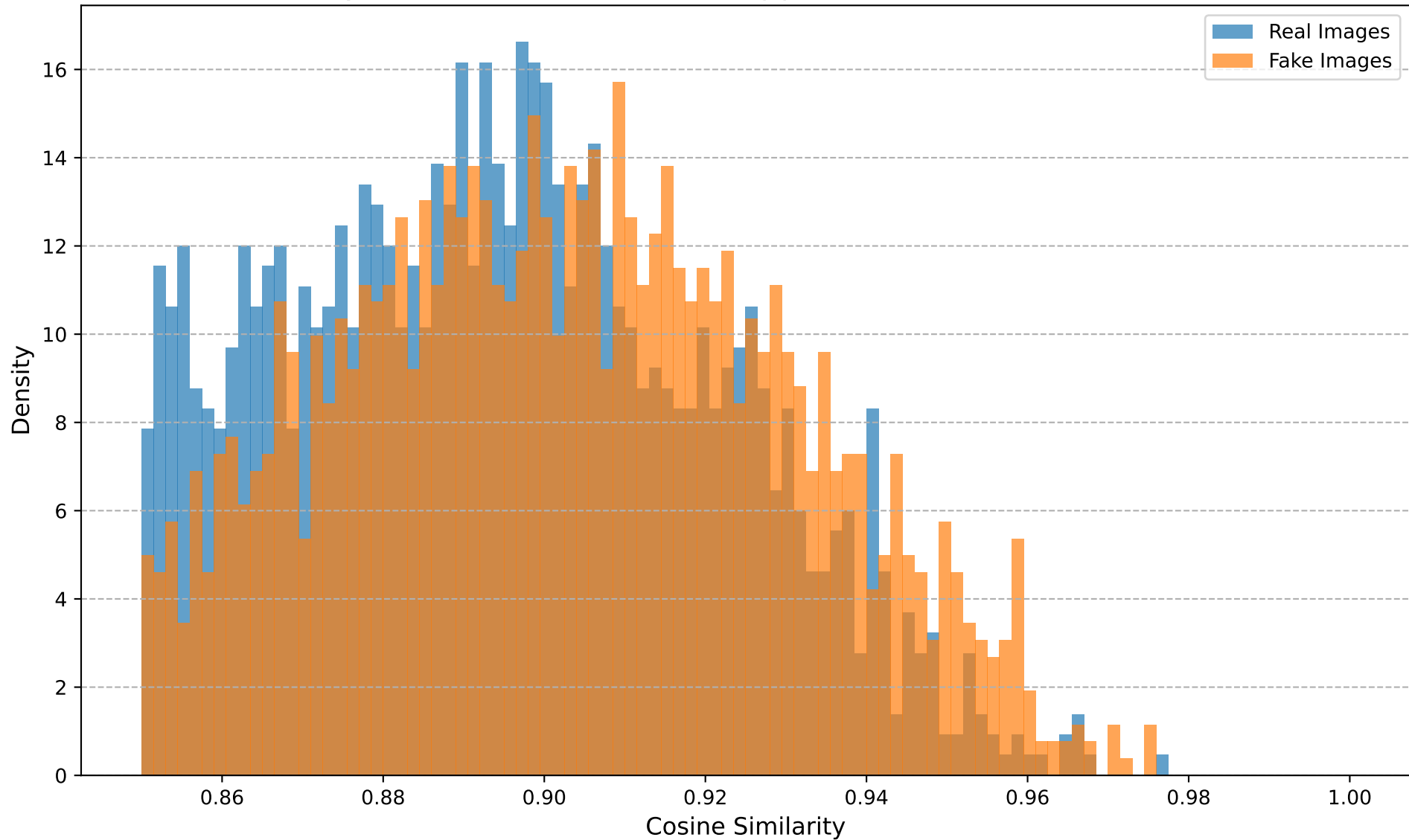
Cosine Similarity Distribution (Dataset: biggan, Transform: Noise, Noise STD=0.1)
