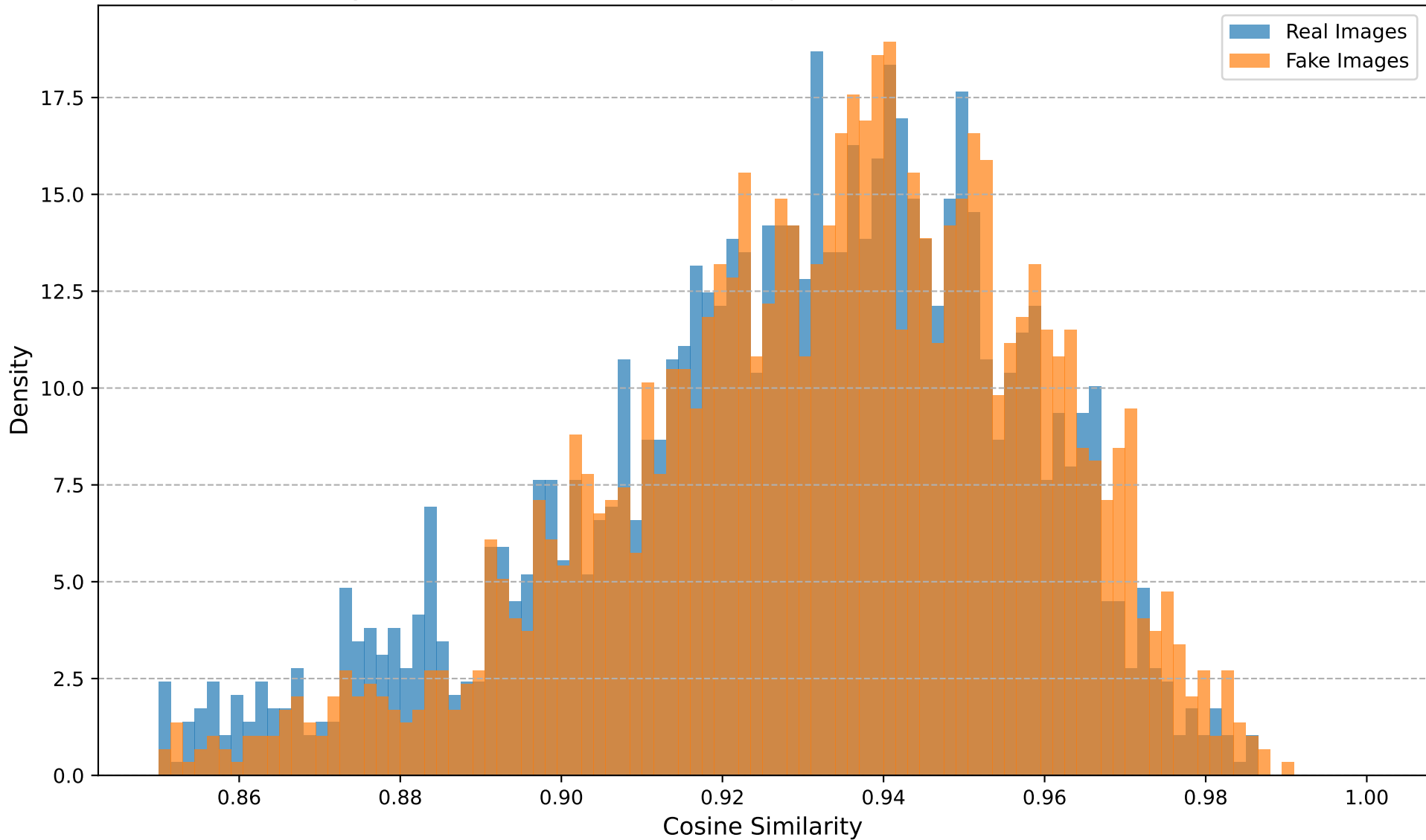
Cosine Similarity Distribution (Dataset: biggan, Transform: Noise, Noise STD=0.05)
