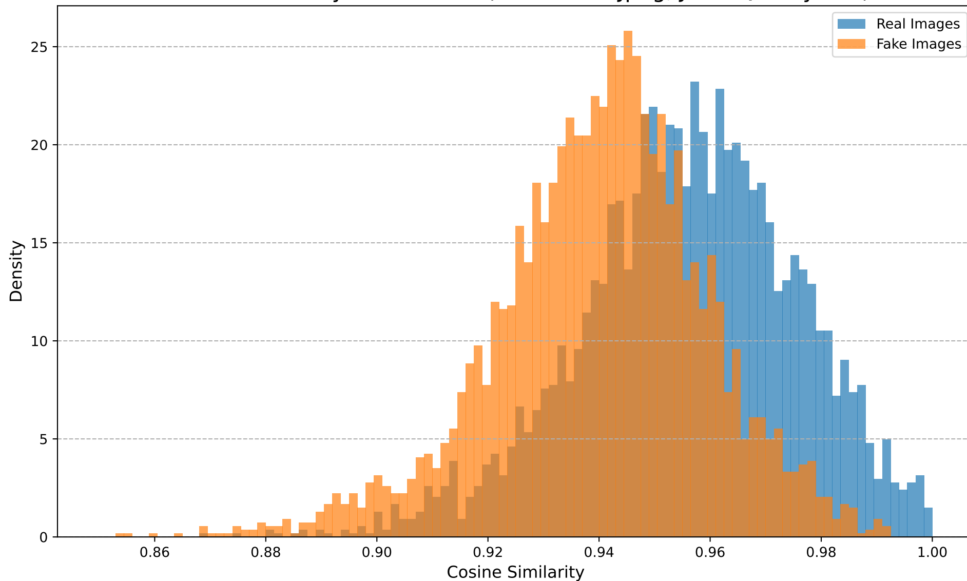
Cosine Similarity Distribution (Transform: jpeg, JPEG Quality=85)
