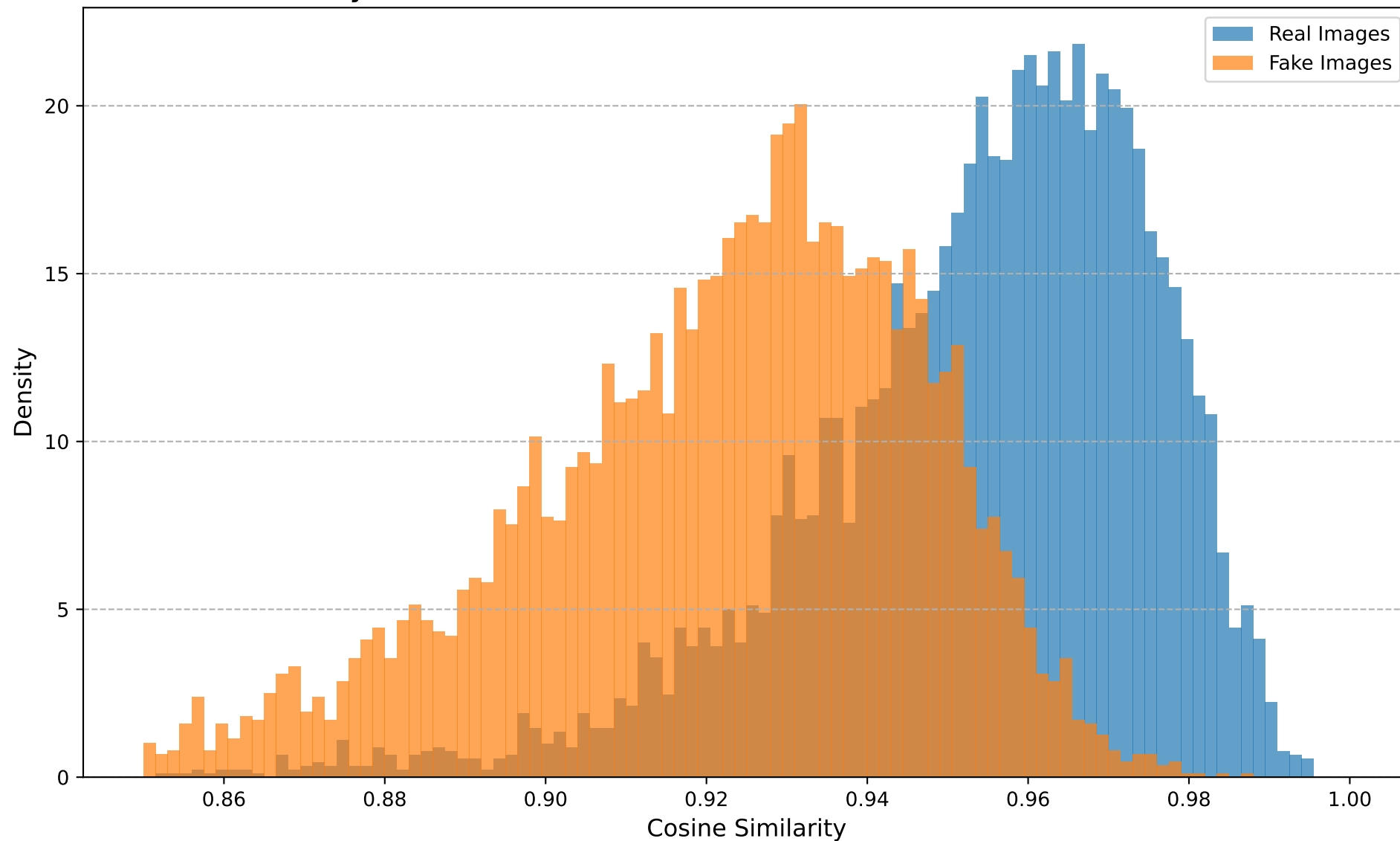
Cosine Similarity Distribution (Dataset: Glide, Transform: Noise, Noise STD=0.03)
