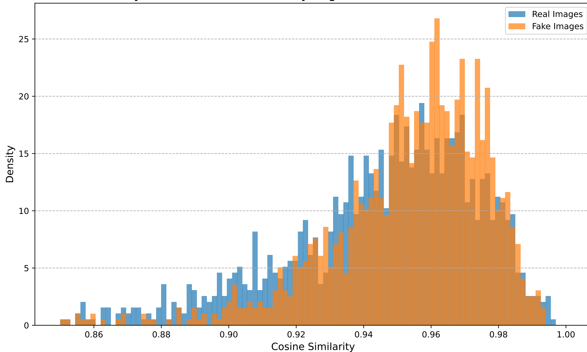
Cosine Similarity Distribution (Dataset: cyclegan, Transform: Noise, Noise STD=0.03)
