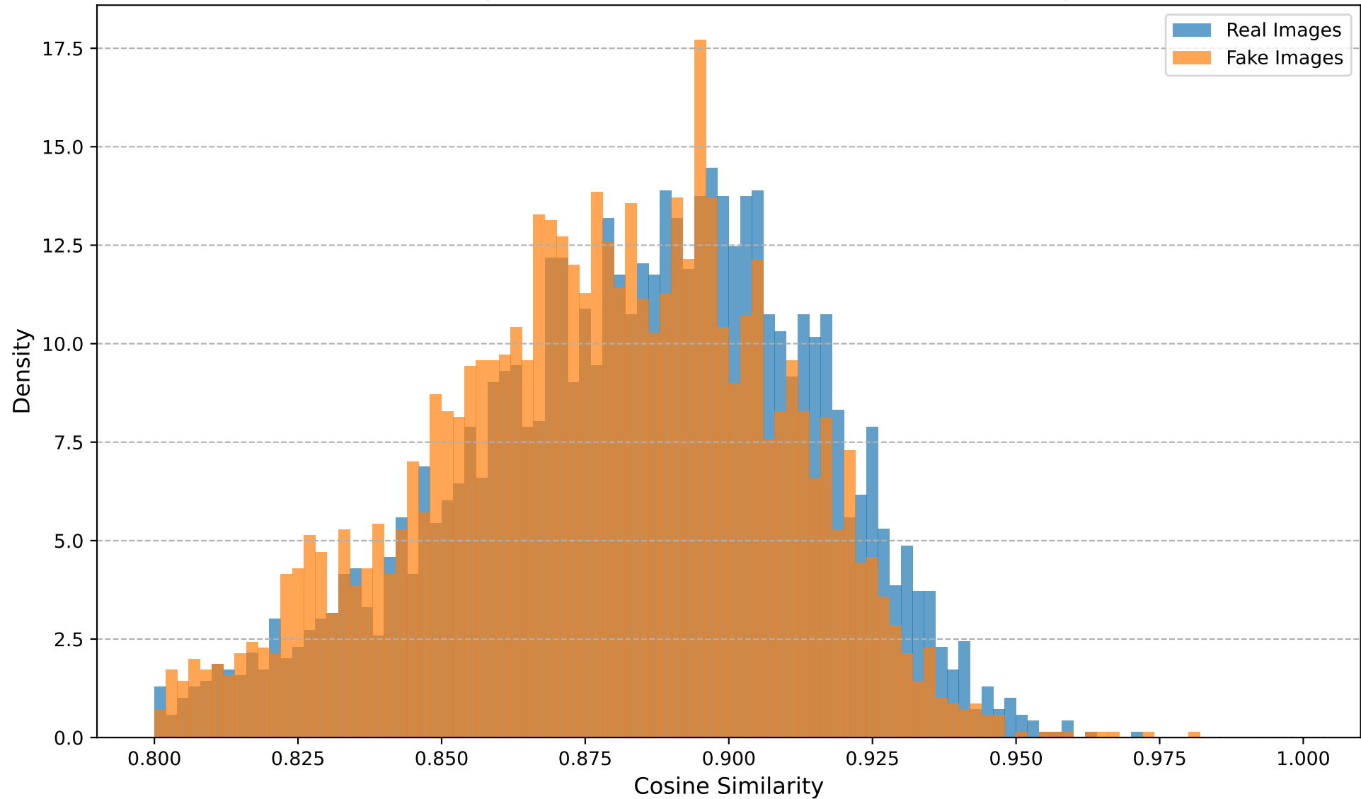
Cosine Similarity Distribution (Transform: Blur, Blur Sigma=1.5)
