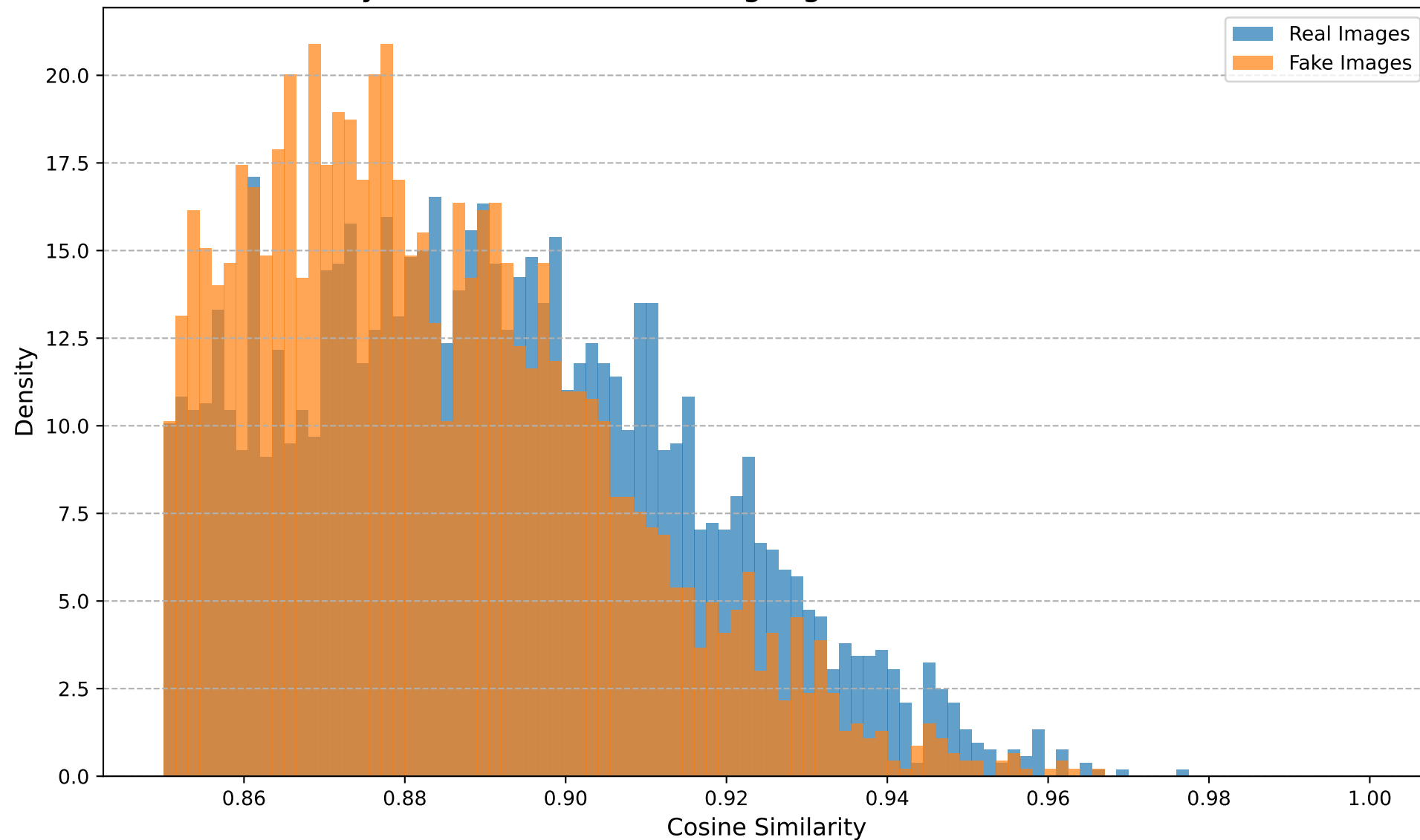
Cosine Similarity Distribution (Dataset: gaugan, Transform: Noise, Noise STD=0.1)
