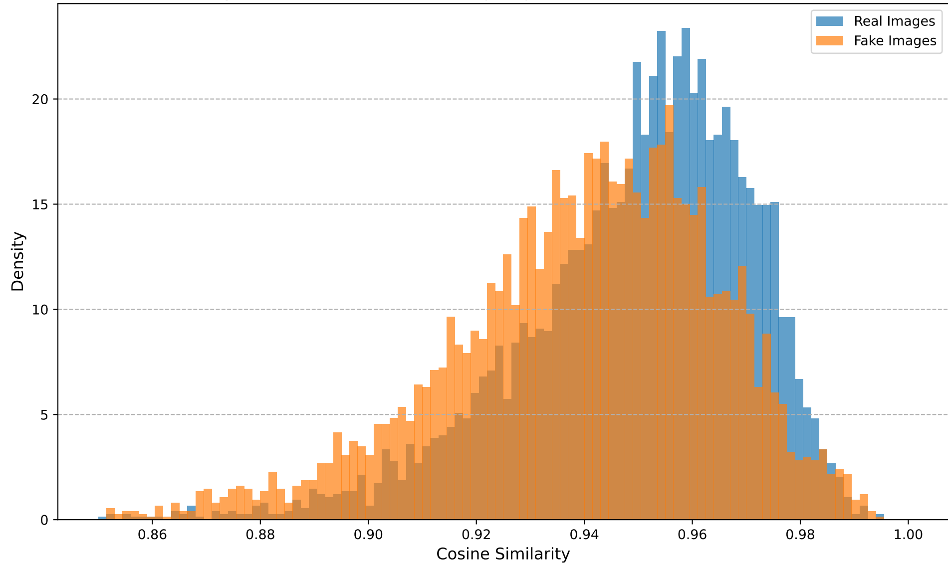
Cosine Similarity Distribution (Dataset: gaugan, Transform: Noise, Noise STD=0.03)
