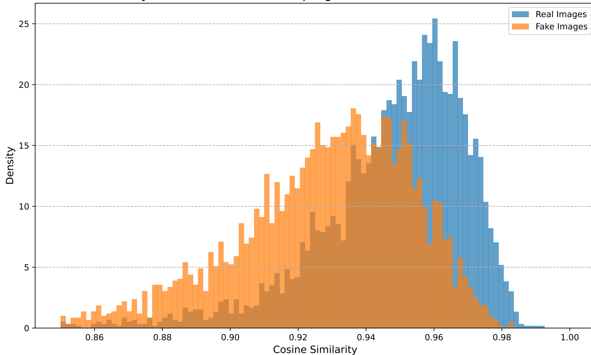
Cosine Similarity Distribution (Dataset: progan, Transform: Noise, Noise STD=0.03)
