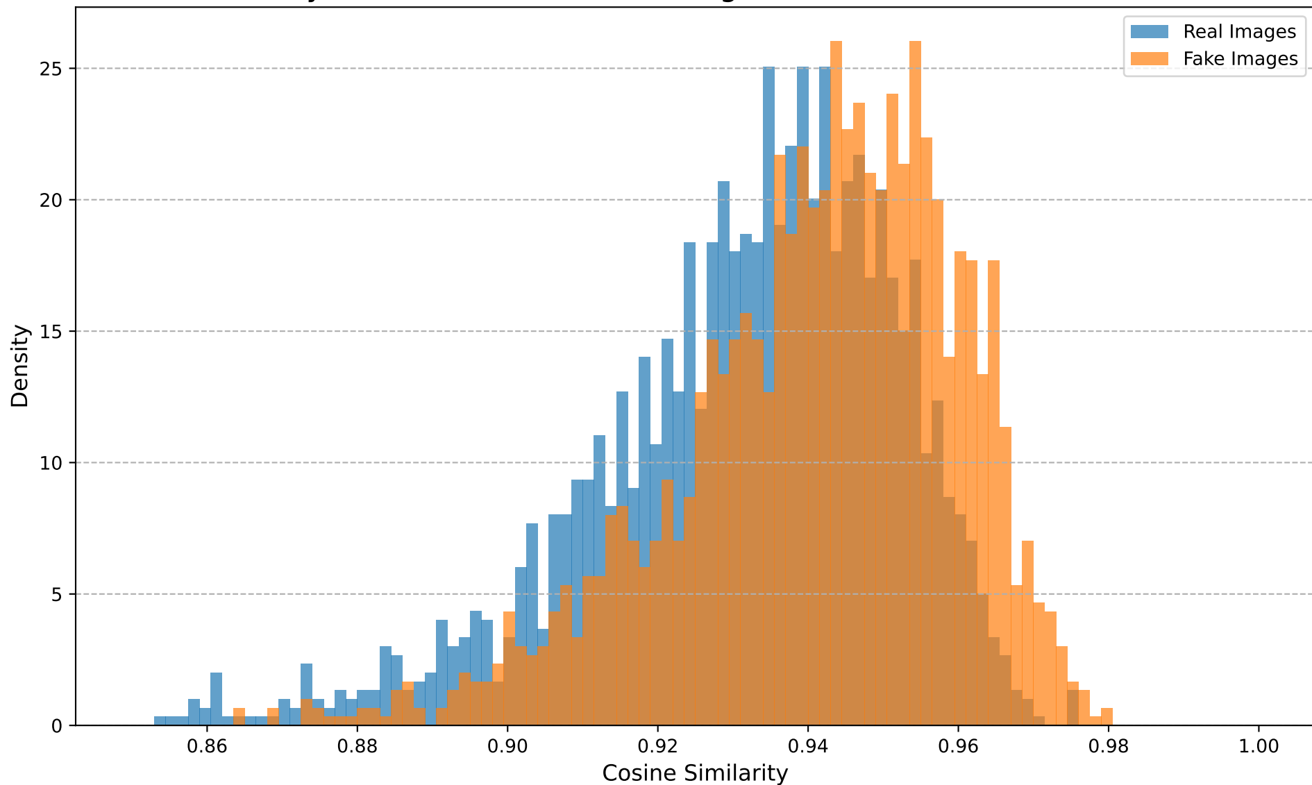
Cosine Similarity Distribution (Dataset: stargan, Transform: Noise, Noise STD=0.03)
