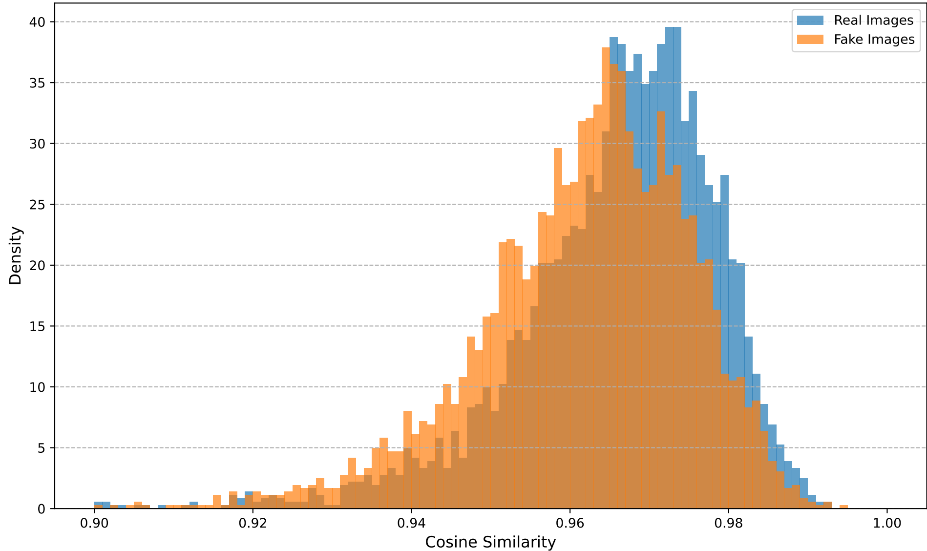
Cosine Similarity Distribution (Transform: Blur, Blur Sigma=0.7)
