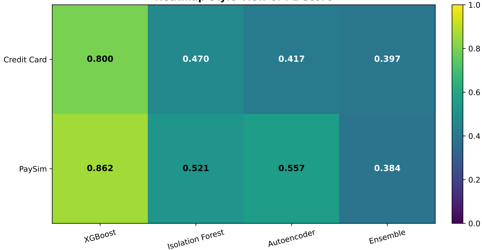
Heatmap-style View of F1-score
