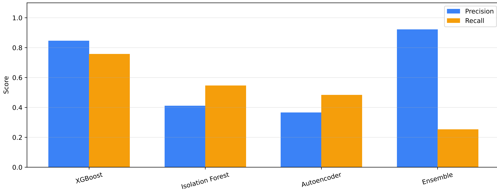
Precision vs Recall — PaySim
