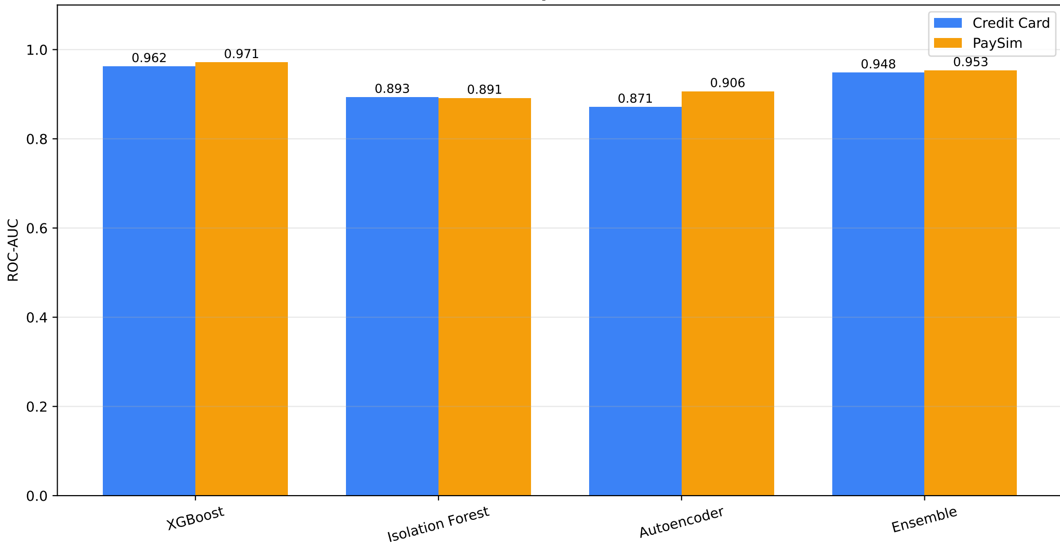
ROC-AUC Comparison of Models
