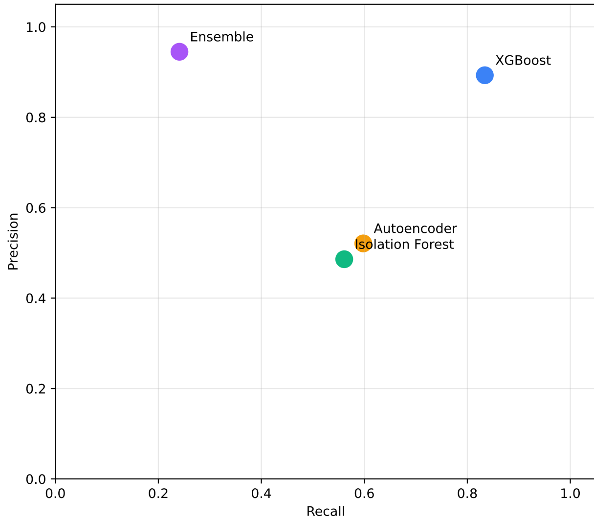
Precision vs Recall Scatter — PaySim
