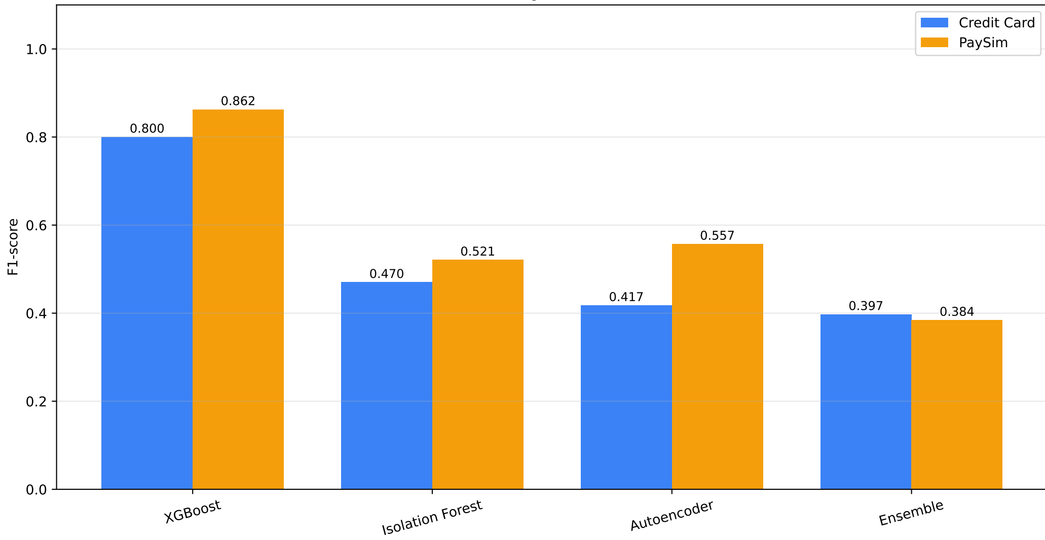
F1-score Comparison of Models
