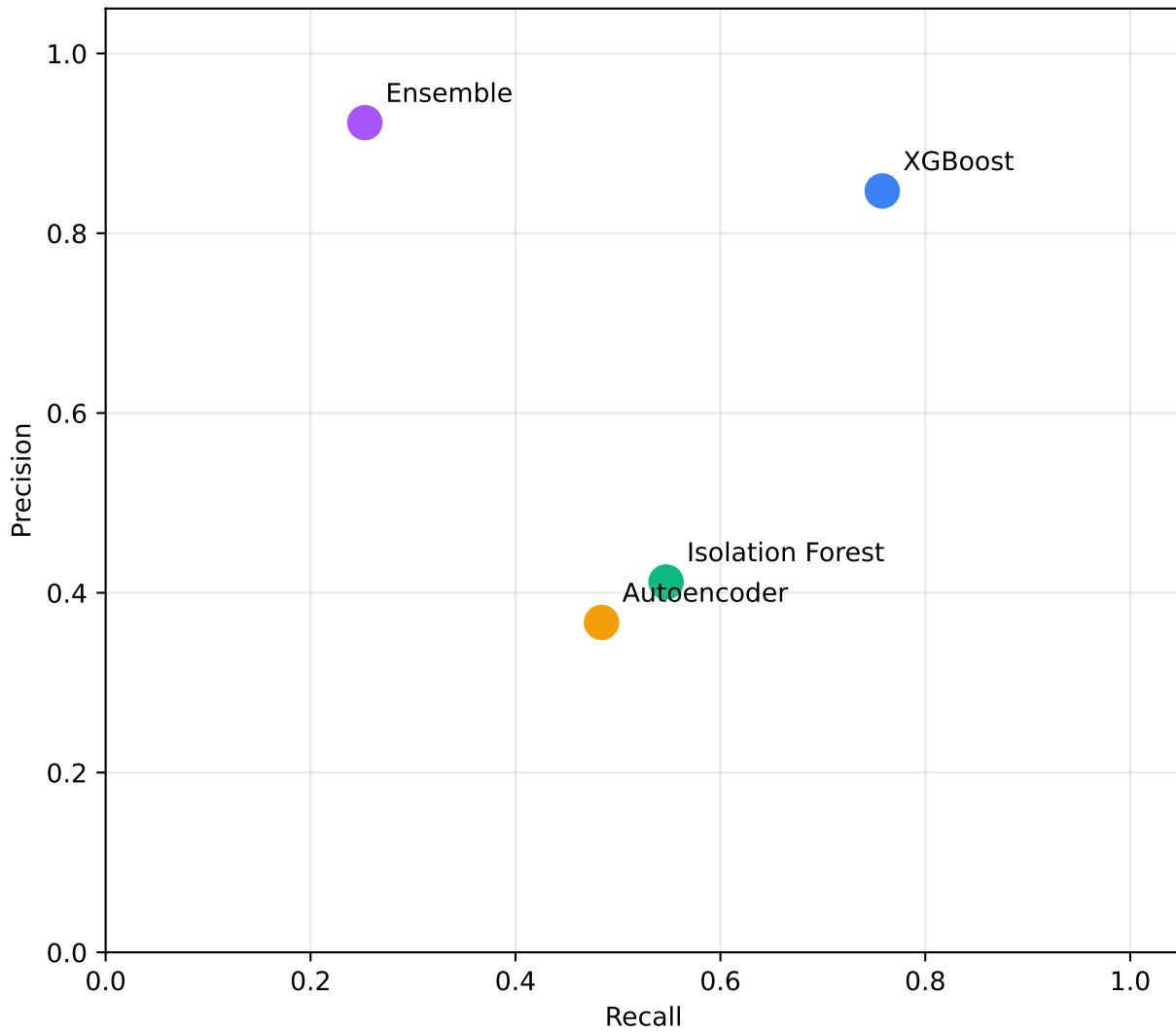
Precision vs Recall Scatter — Credit Card
