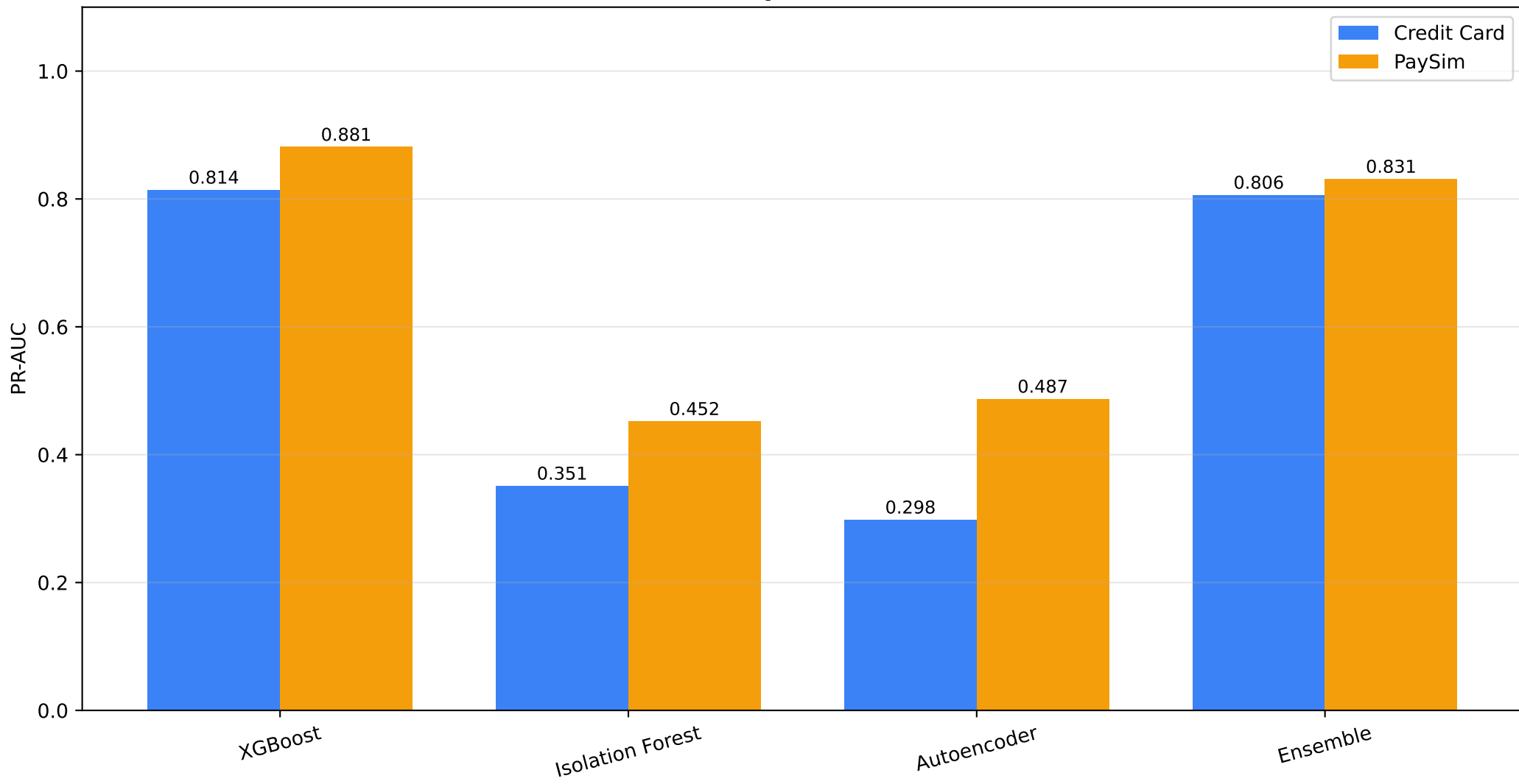
PR-AUC Comparison of Models
