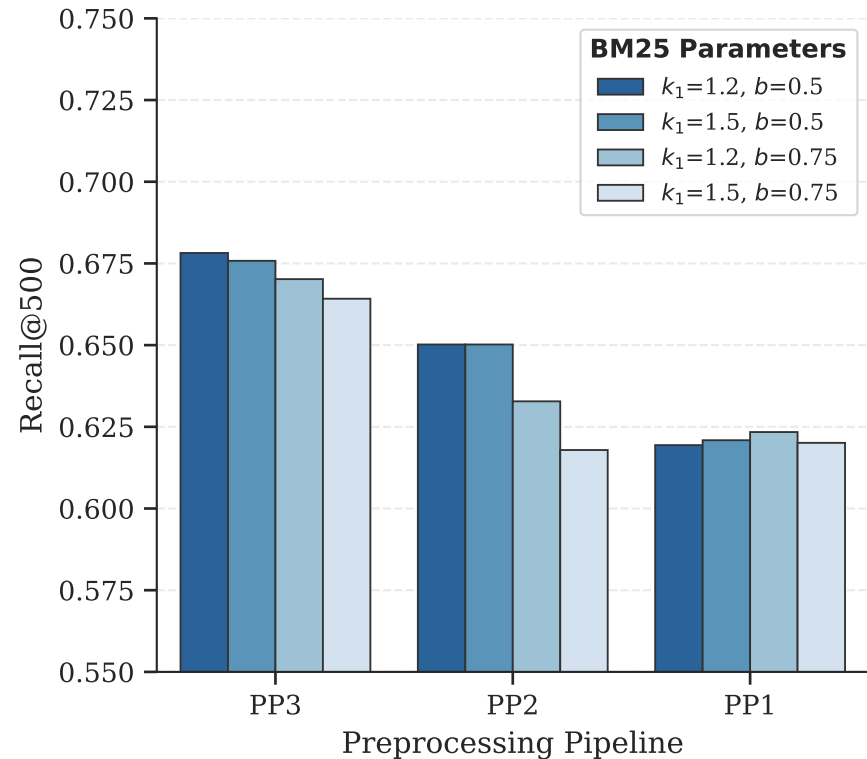
(a) IMPACT OF PREPROCESSING
