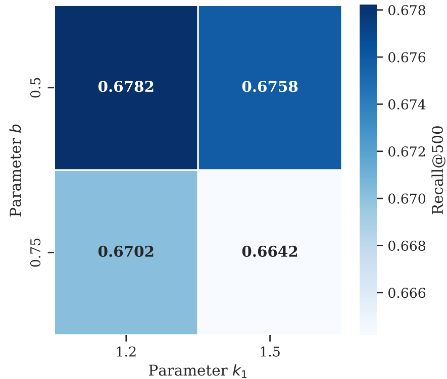
(b) HYPERPARAMETER SEARCH
