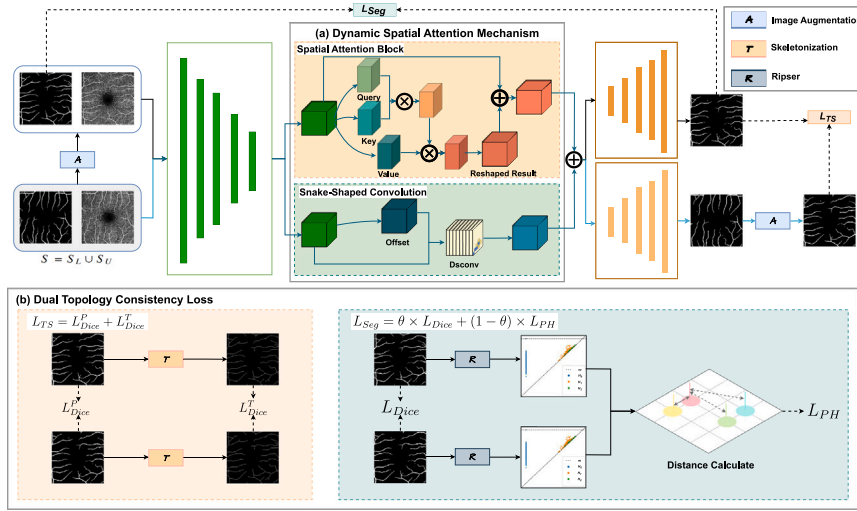
Fig. 2. The overview of the proposed DSDC-NET architecture. DSDC-NET comprises two main components: (a) Dynamic Spatial Attention Mechanism, enhancing the capacity to extract spatial information while focusing on elongated and curved local features, thus reducing false positives; and (b) Dual Topological Consistency Loss, improving the network proficiency in learning the structural hierarchy and branching pattern of vessel system, increasing the likelihood of accurate major vessel segmentation and mitigating false positives from insufficient structural learning. We use three lines, each ranging in colour from dark to light, to distinguish the data flow of the enhanced image, the whole image, and the original image.
