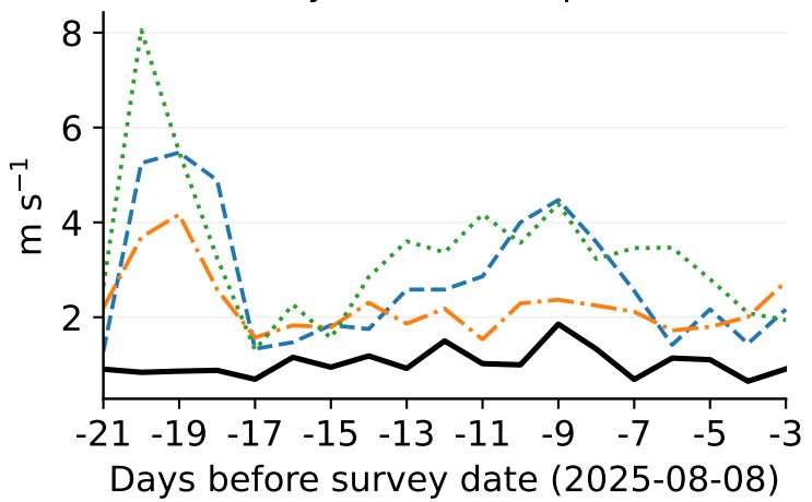
Daily mean wind speed
