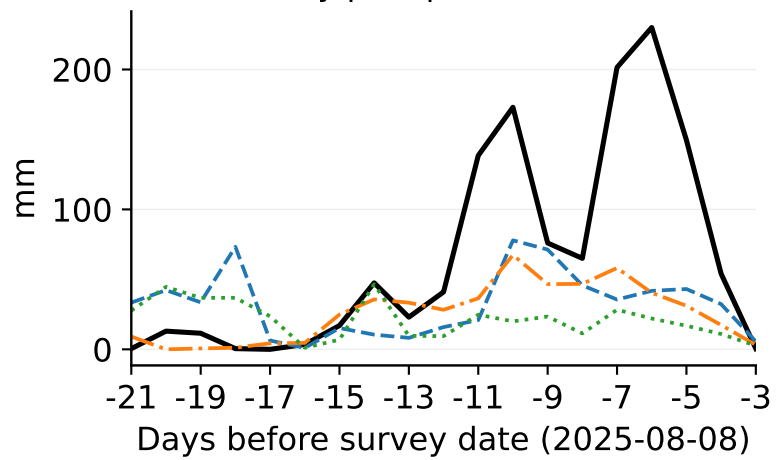
Daily precipitation total
