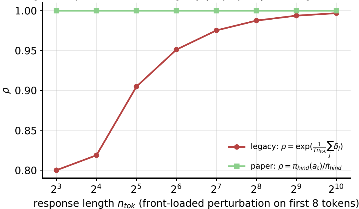
Longer responses inflate legacy \rho ; paper \rho is length-invariant
