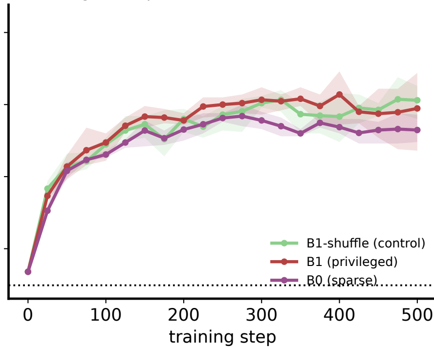
(b) Progress-supervision triad (RQ3), 3 seeds/arm
