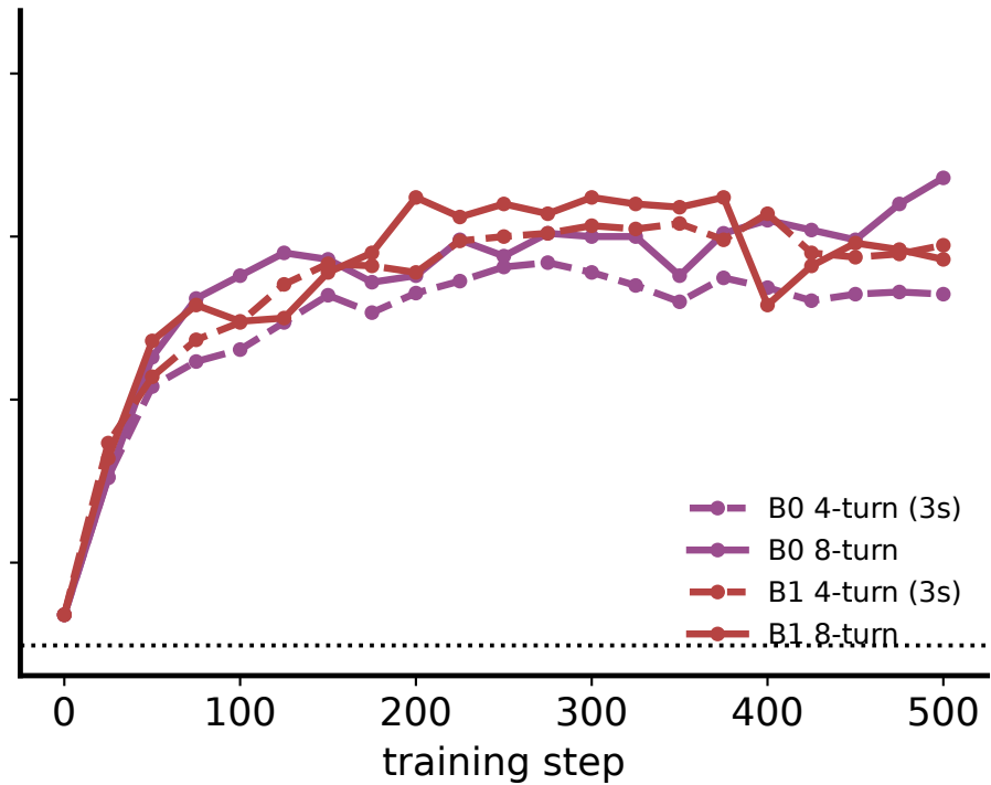
(c) Horizon stress: 4-turn vs 8-turn (RQ4)
