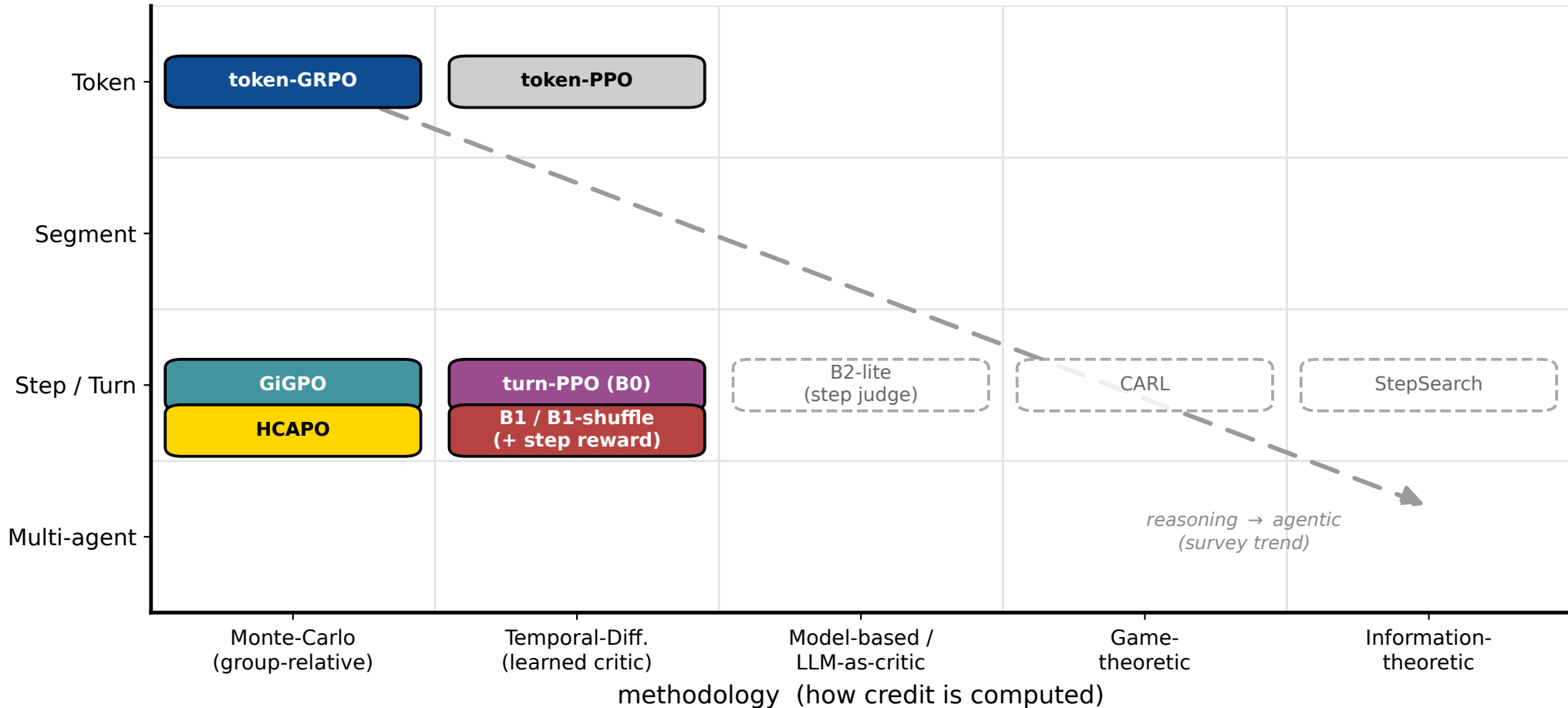
F1 — Wave-1 arms on the credit-assignment taxonomy grid (filled = run; dashed grey = second-wave roadmap)
