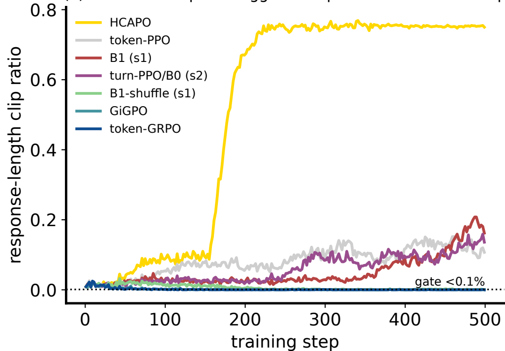
(a) Truncation tripwire: aggressive per-turn credit blows up
