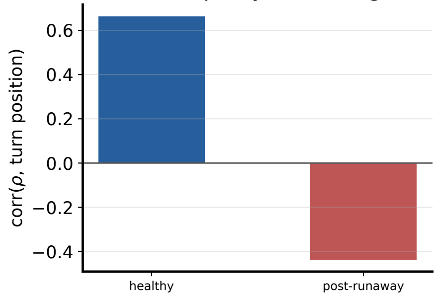
Position preference FLIPS with the policy's own length
