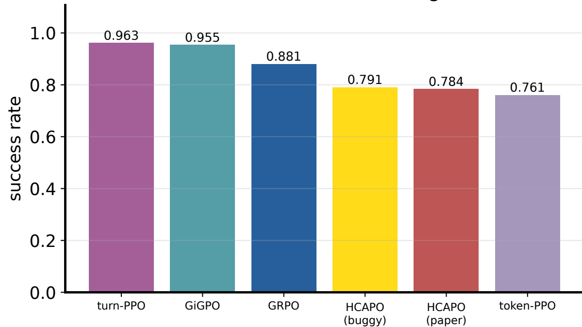
AlfWorld (1.7B, unseen 134 games)
