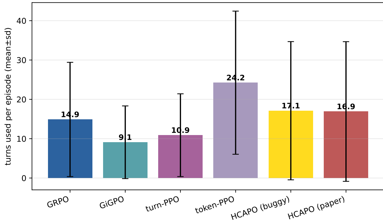
AlfWorld — trajectory length (unseen 134)
