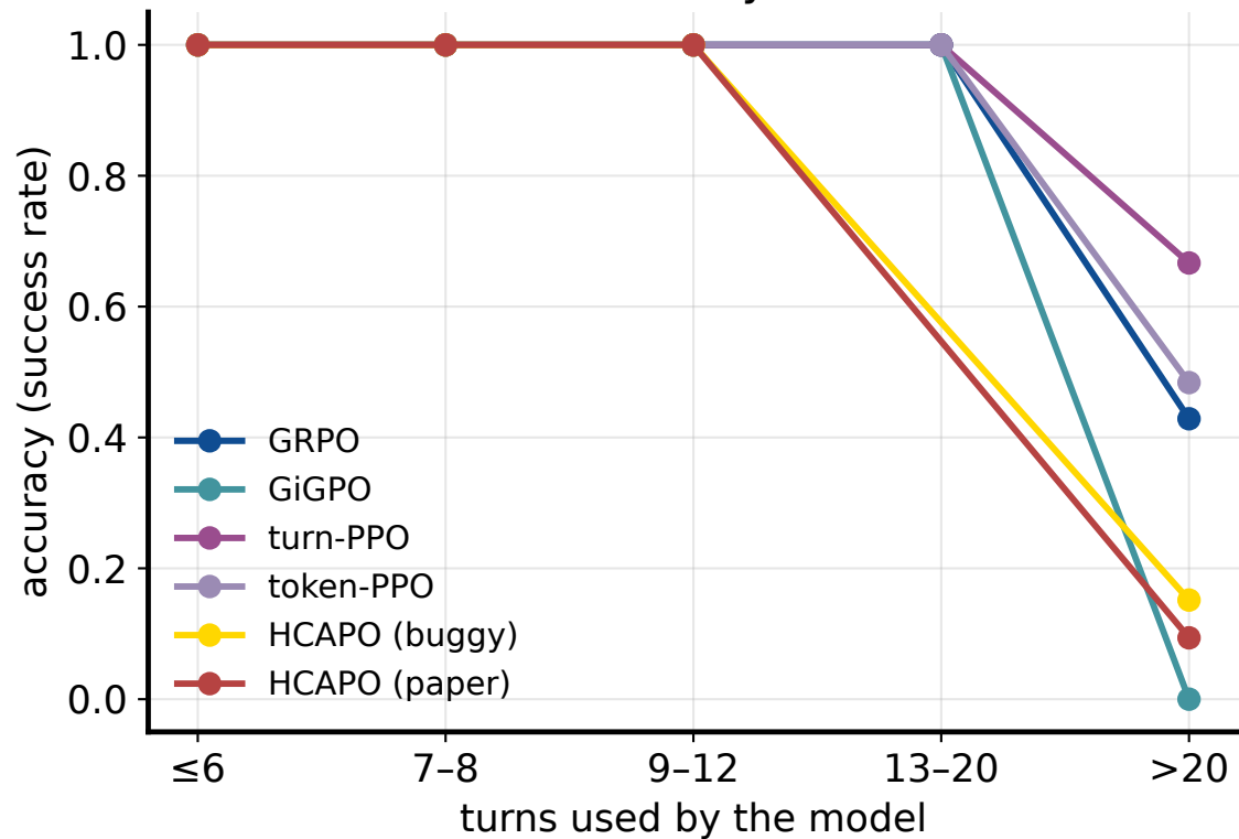
AlfWorld — accuracy vs turns used
