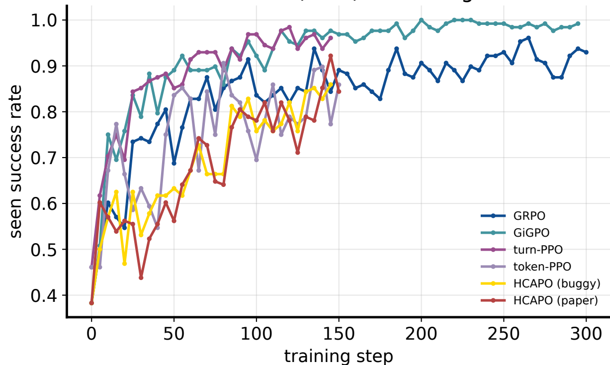
AlfWorld (1.7B) — training
