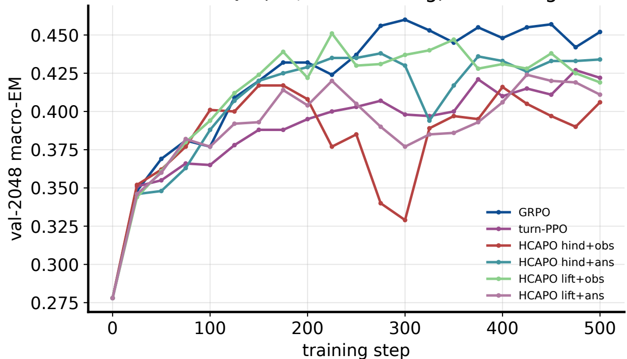
SearchQA (4B, non-thinking) — training
