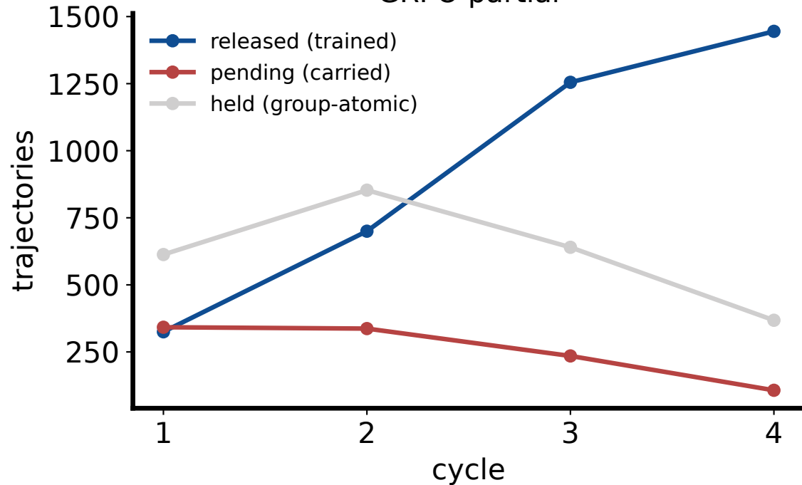
GRPO partial
