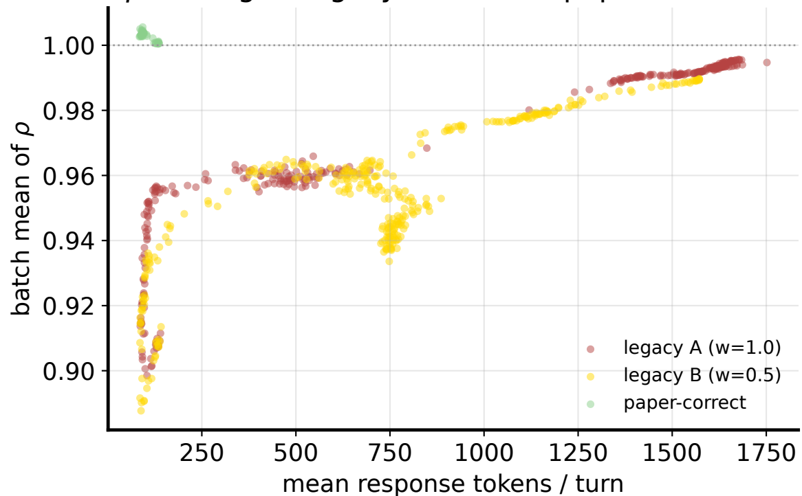
\rho vs length: legacy co-moves, paper does not
