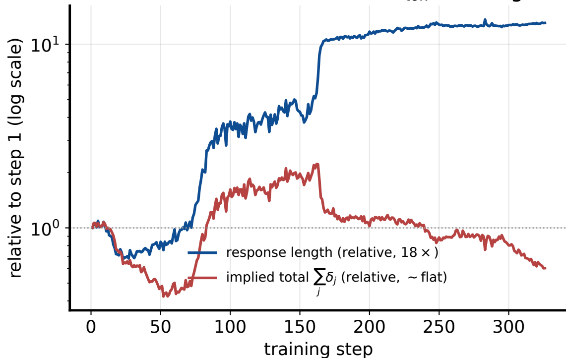
numerator saturates while the /n_{tok} divisor grows
