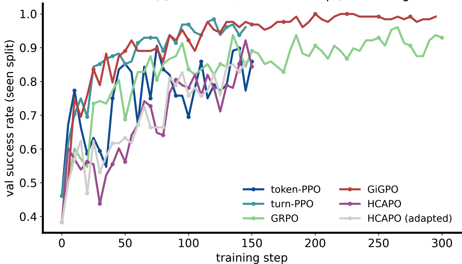
ALFWorld (Qwen3-1.7B, ReAct transcript) — training
