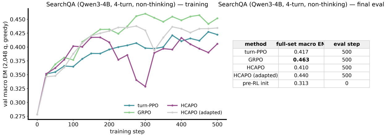
Figure 1: SearchQA, Qwen3-4B, 4-turn non-thinking, 500 steps. Left: greedy validation macro-EM (2,048 questions) every 25 steps. Right: full-set (51,713-question) macro EM at step 500, best non-baseline value in bold. token-PPO and GiGPO curves/rows appear when their arms complete.
