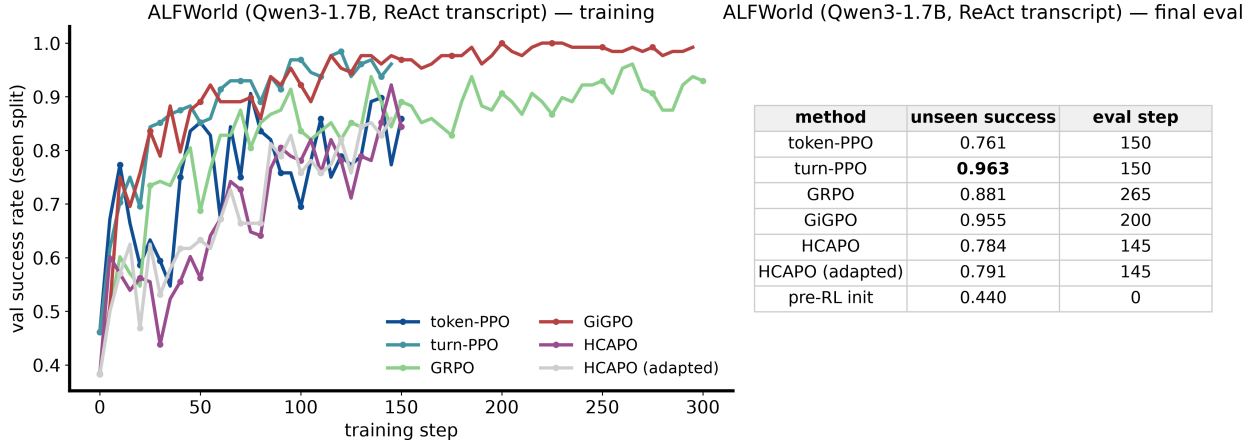
Figure 2: ALFWorld, Qwen3-1.7B from replay-BC . Left: seen-split validation success (logged every 5 steps; PPO/HCAPO arms trained 150 steps, GRPO/GiGPO 300 — budgets follow the original campaign). Right: unseen 134-game success at each method’s best checkpoint.
