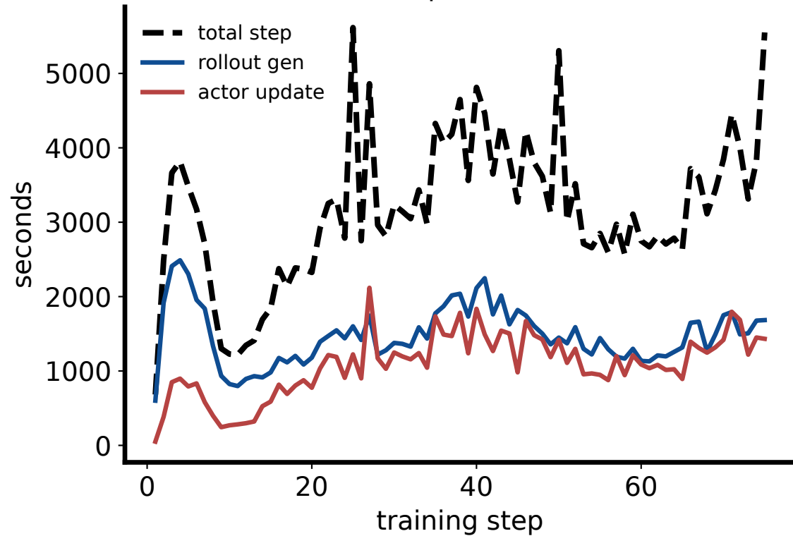
GRPO (75 steps, 1×H100 node)
