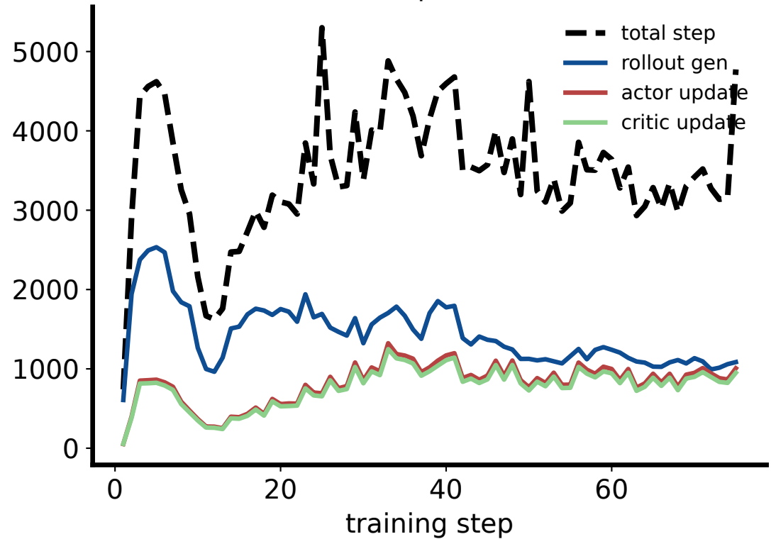
turn-PPO (75 steps, 1×H100 node)
