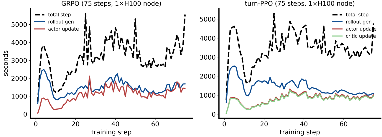
Figure 1: Per-step phase times across training. GRPO’s step time grows 1.6\times (2,447s first-10 \rightarrow 3,885s last-10): its policy inflates to \sim 17 turns and per-turn responses shrink, so update + logprob costs triple while gen stays flat. turn-PPO is flat end-to-end (3,395s \rightarrow 3,393s): the critic steers toward \sim 7.5 -turn episodes, gen falls from 1,930s to 1,067s, paying for the critic’s own \sim 27\% overhead. Spikes are val/checkpoint steps.
