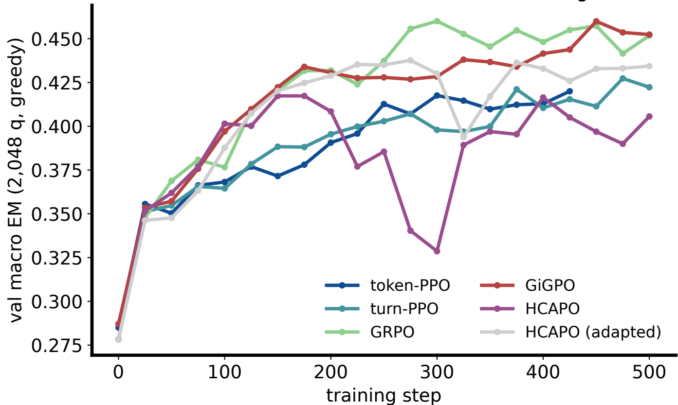
SearchQA (Qwen3-4B, 4-turn, non-thinking)
