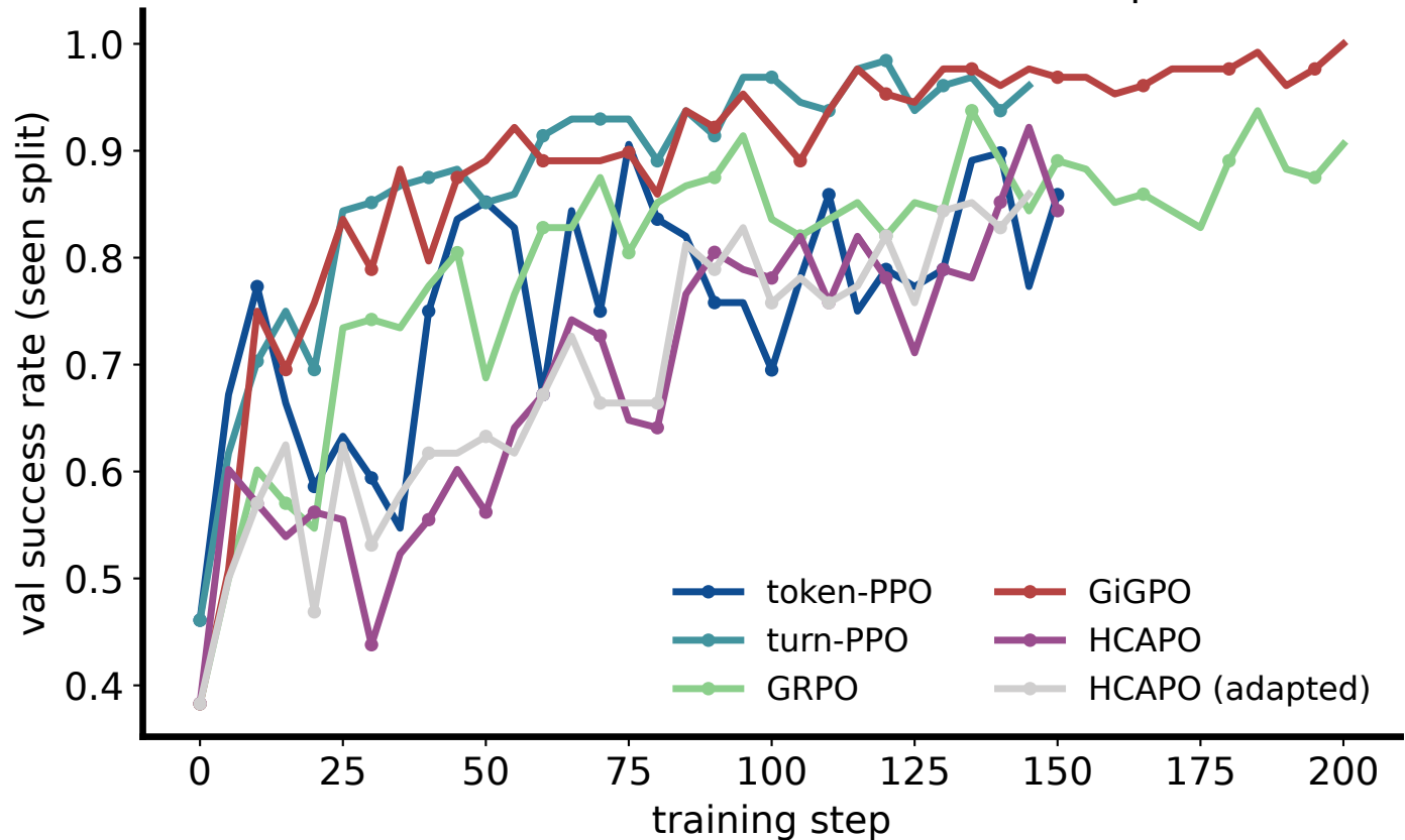
ALFWorld (Qwen3-1.7B, ReAct transcript)
