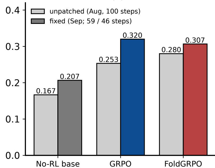
Greedy pass@1
