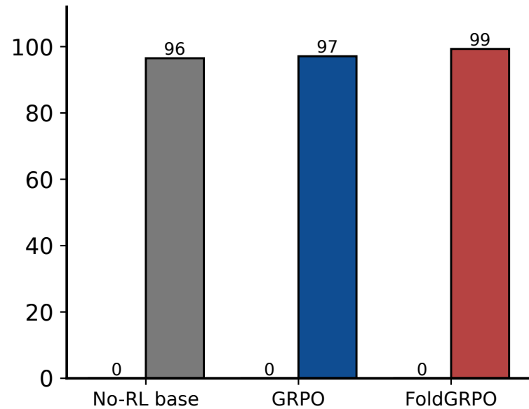
Intact observations (%)
