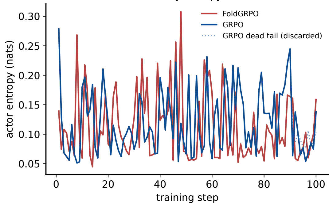
Policy entropy
