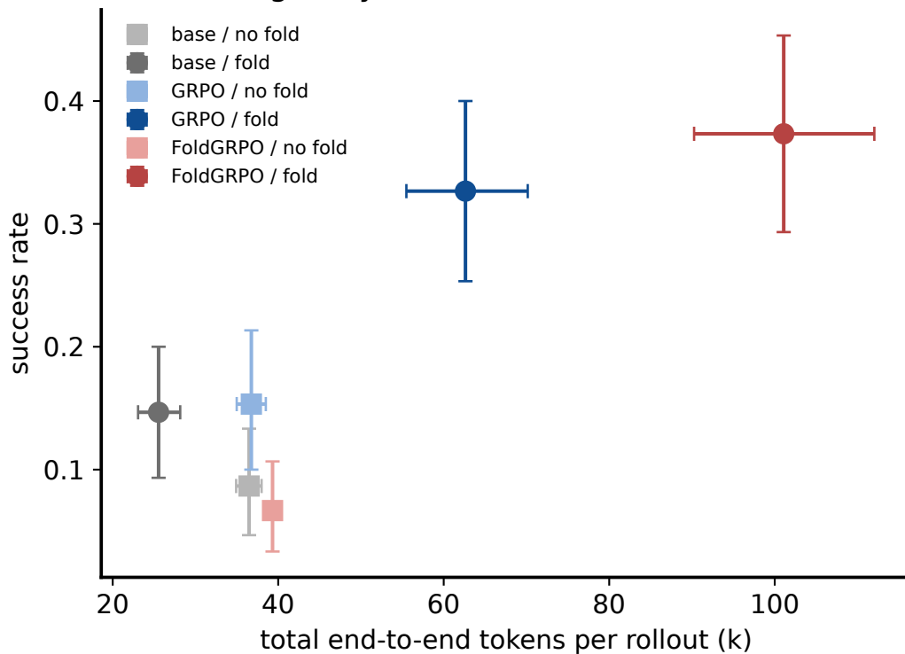
greedy: solved-within-budget
