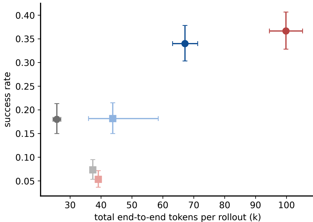
t1n4: solved-within-budget
