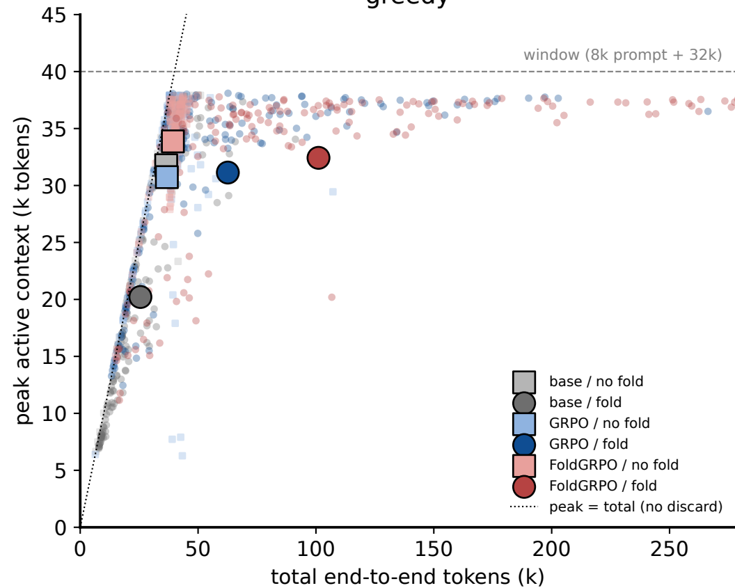
greedy
