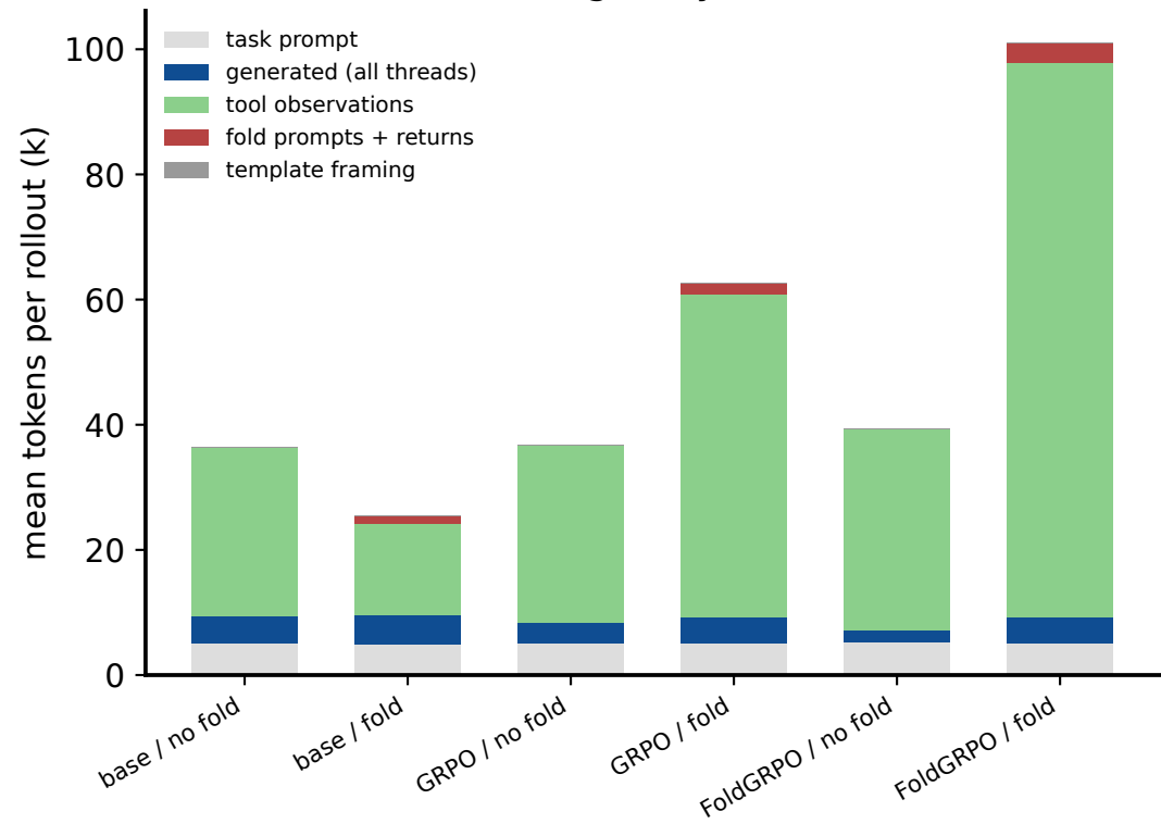
greedy
