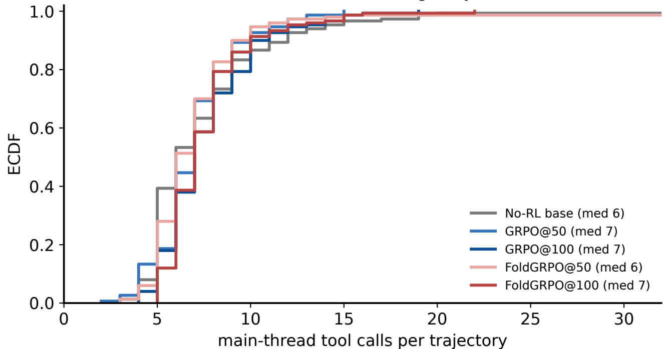
Main-thread tool-call distribution (greedy, n=150/arm)
