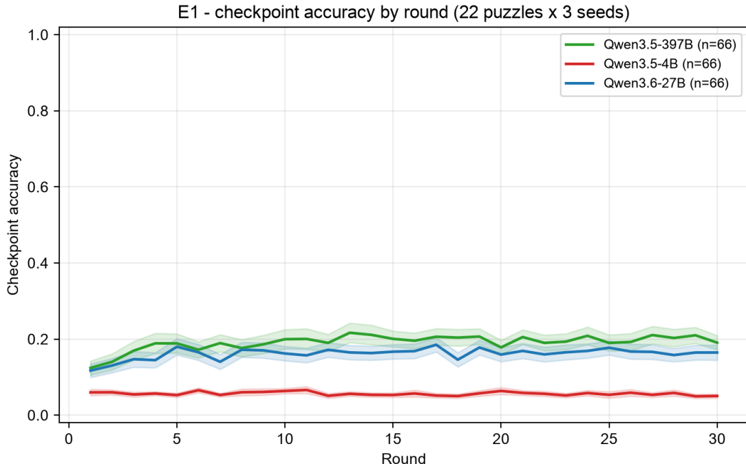
Figure 1: E1: mean checkpoint accuracy by round (22 puzzles \times 3 seeds per model), on the full 0–1 outcome range so that flatness reads as flat. Gains exist only before round \sim 10 and only at scale; the 4B curve never moves.
