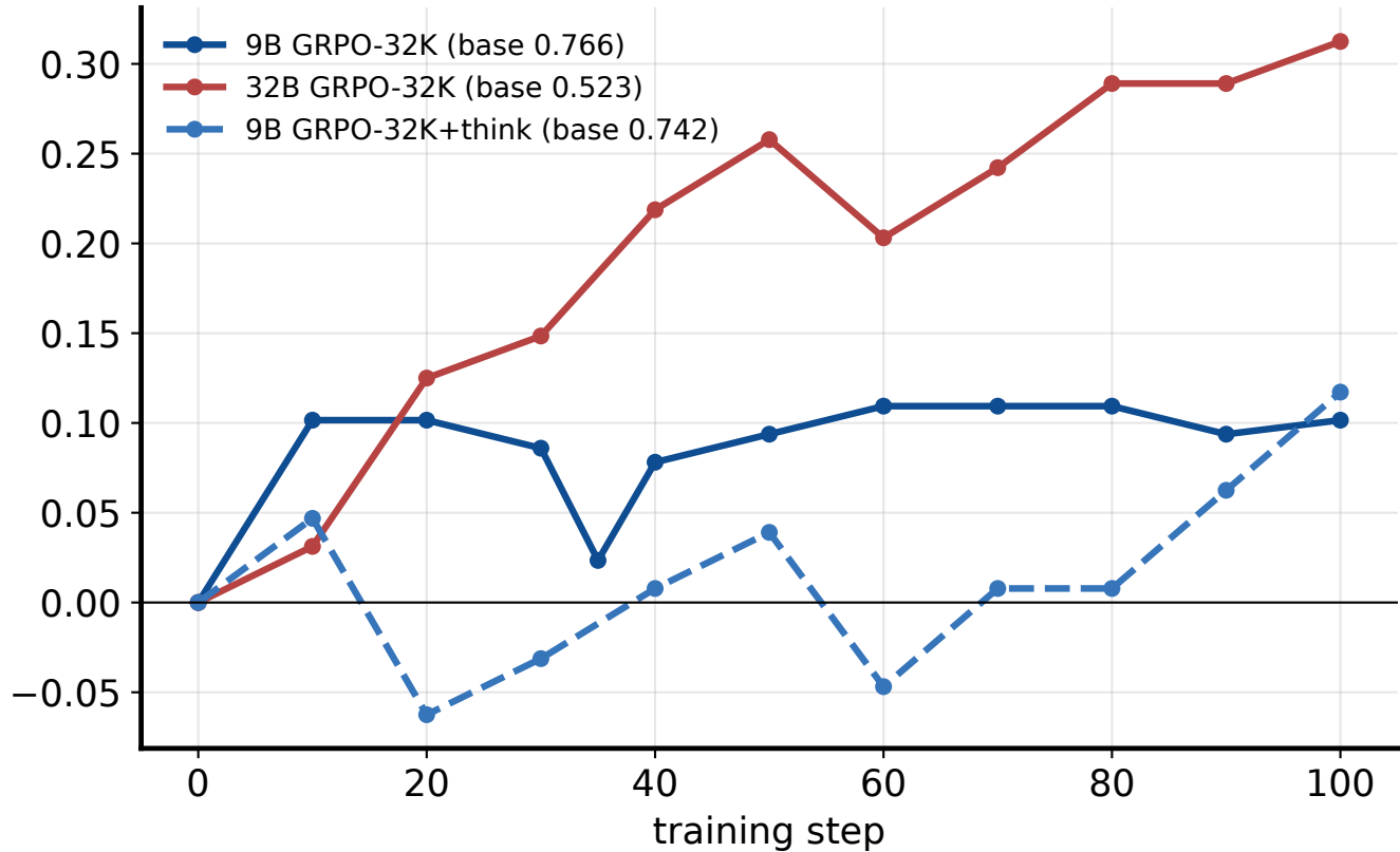
accuracy gain over step 0
