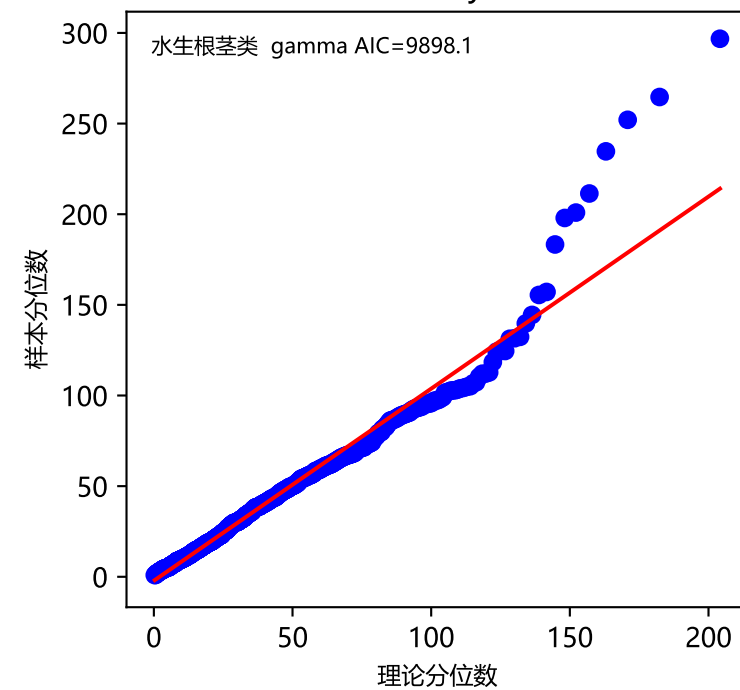
Probability Plot
