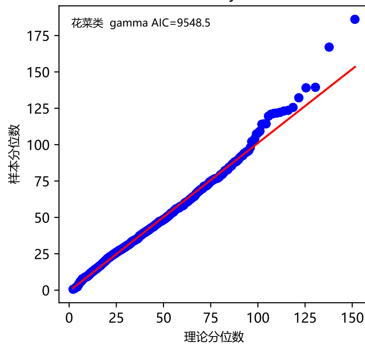
Probability Plot
