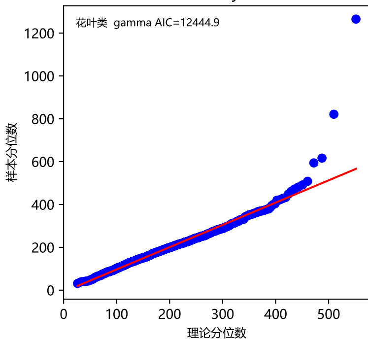
Probability Plot
