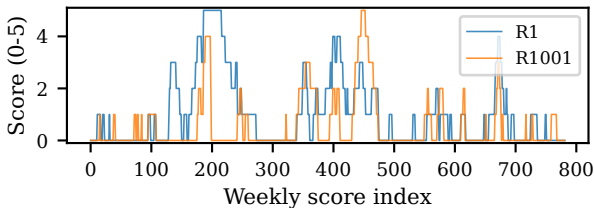
(b) Two example regions
