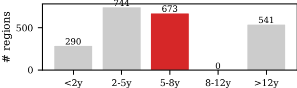
(c) Multi-year cycle coverage
