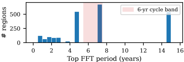
(a) FFT top-period distribution
