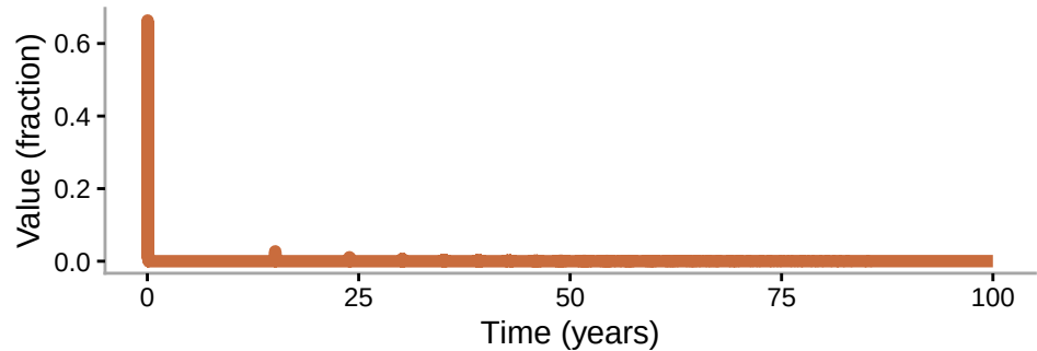
Infectious proportion (i)
