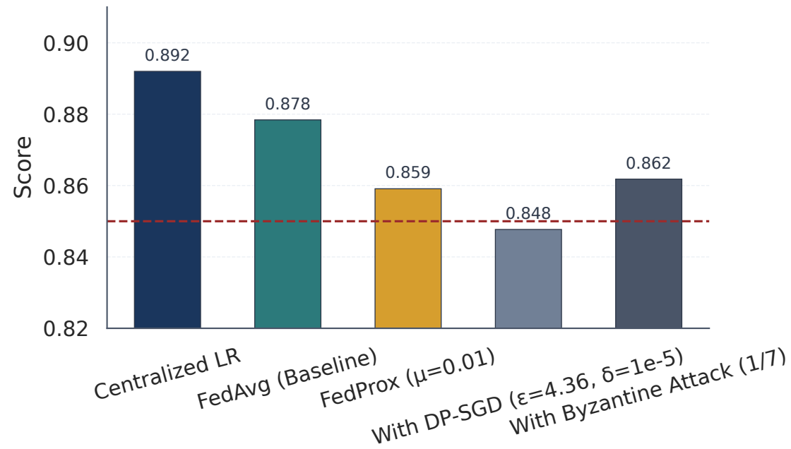
Validation AUROC
