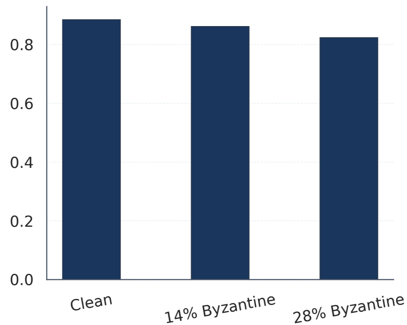
Validation AUROC
