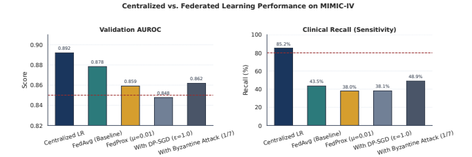
Fig. 7. Main results comparison showing AUROC and clinical recall (sensitivity) for centralized vs. federated learning under Non-IID conditions. DP-SGD values are reported at the Platt-calibrated threshold (0.39); see Table I for full details.
