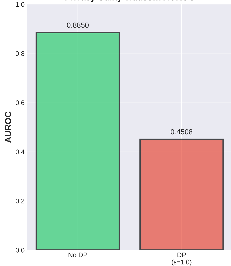
Privacy-Utility Tradeoff: AUROC
