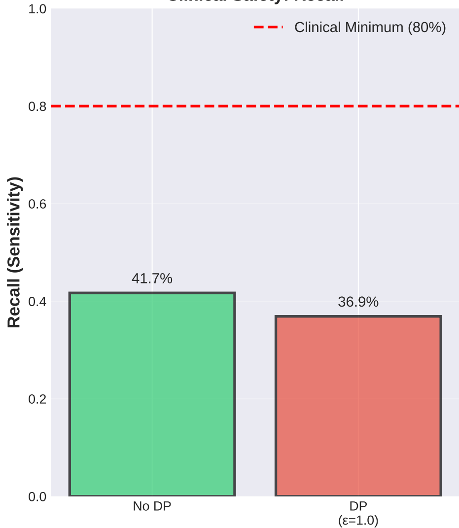
Clinical Safety: Recall
