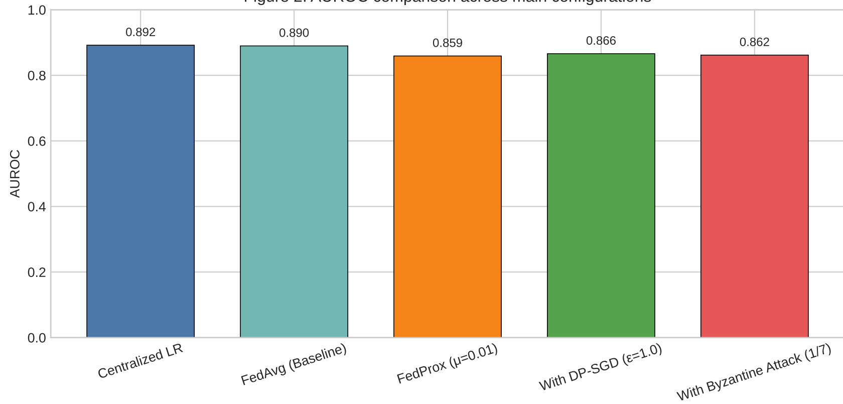
Figure 2. AUROC comparison across main configurations
