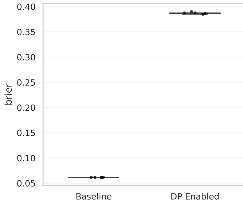
Brier Score
