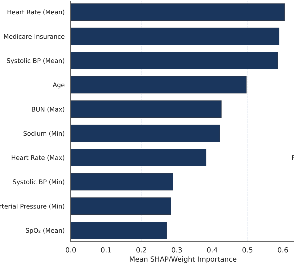
Mean Feature Importance Across Sites
