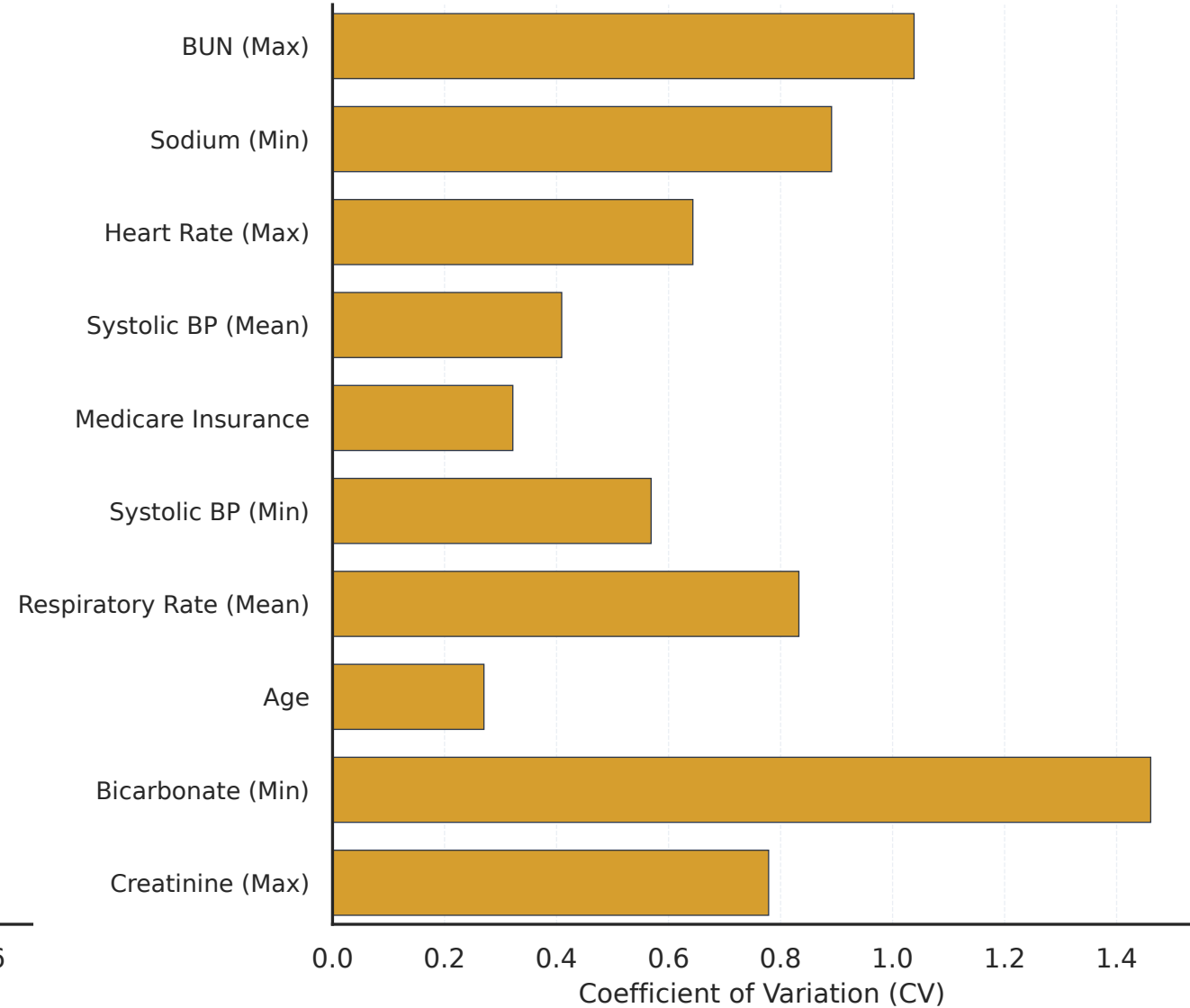
High-Drift Clinical Features
