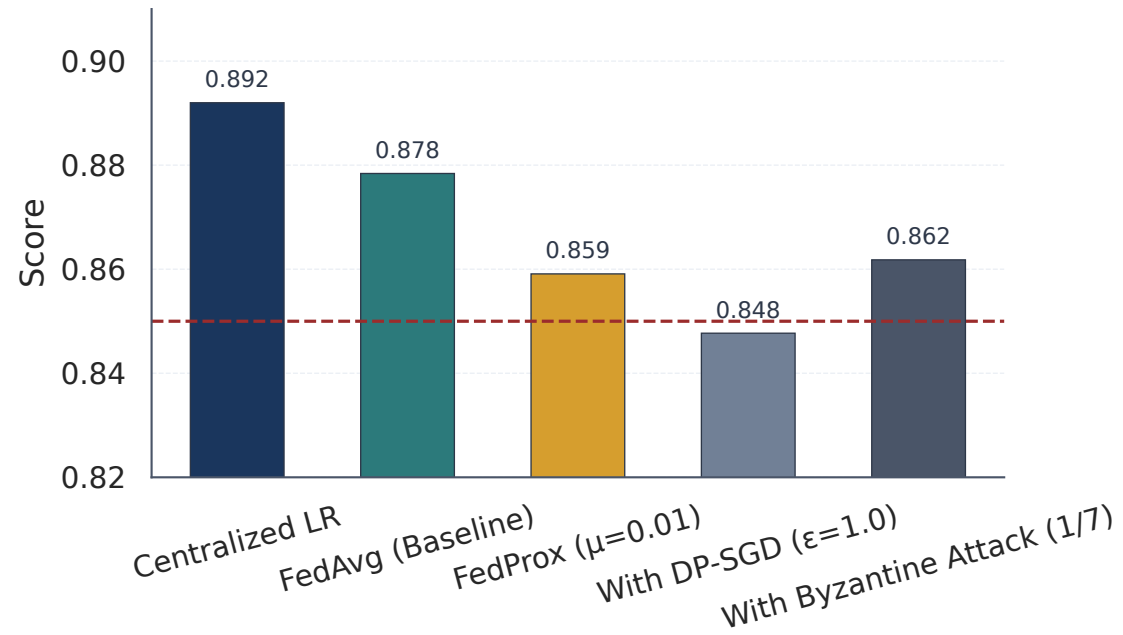
Validation AUROC
