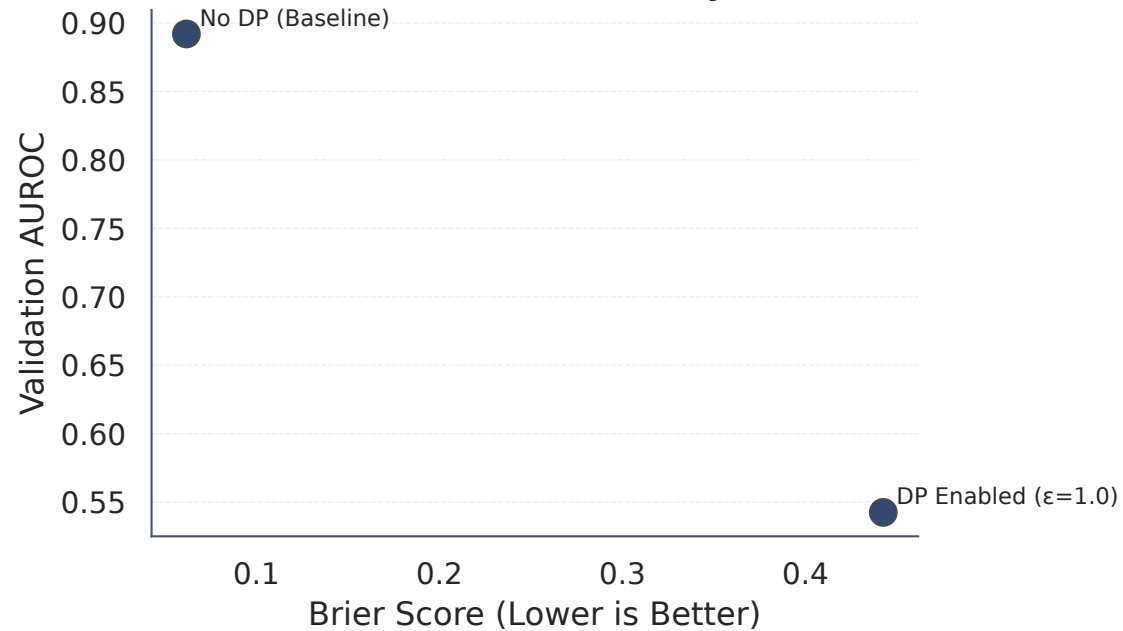
Brier Score vs. Utility
