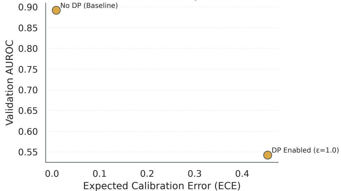
ECE vs. Utility
