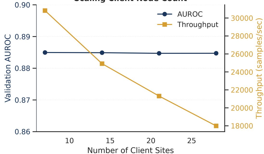
Scaling Client Node Count
