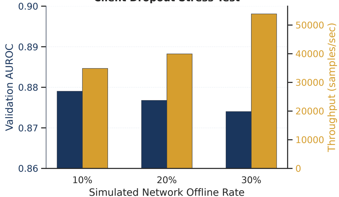
Client Dropout Stress Test
