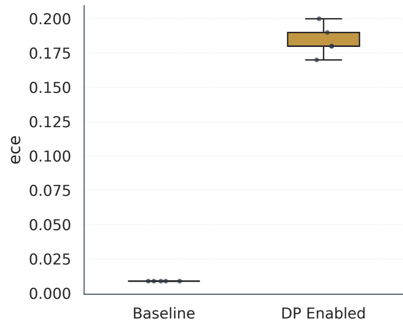
ECE (Calibration Error)
