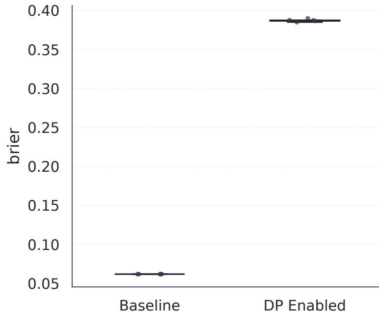
Brier Score (Calibration)
