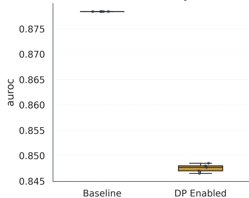
AUROC (Utility)
