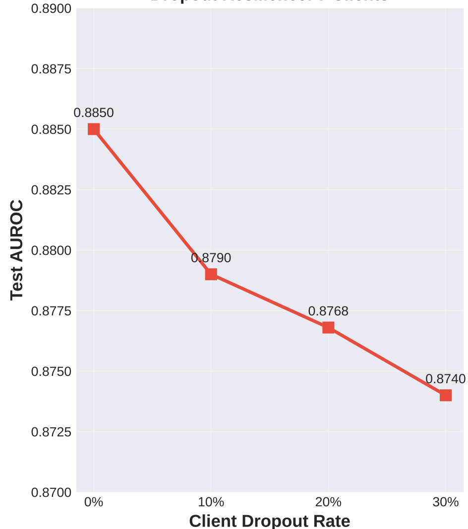
Dropout Resilience: 7 Clients
