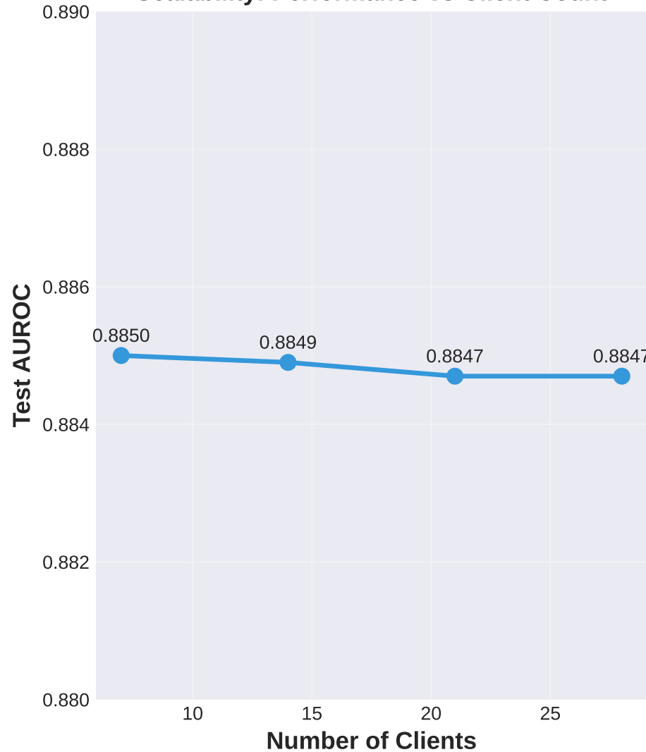
Scalability: Performance vs Client Count
