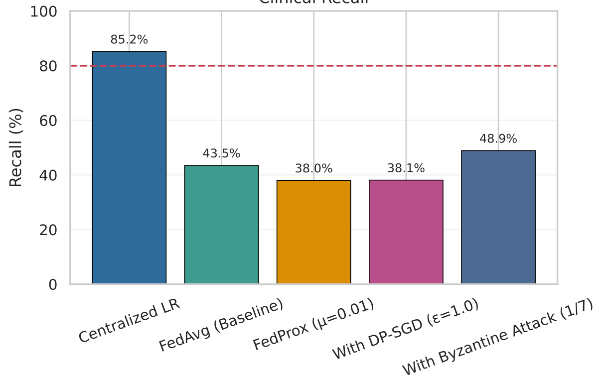
Clinical Recall
