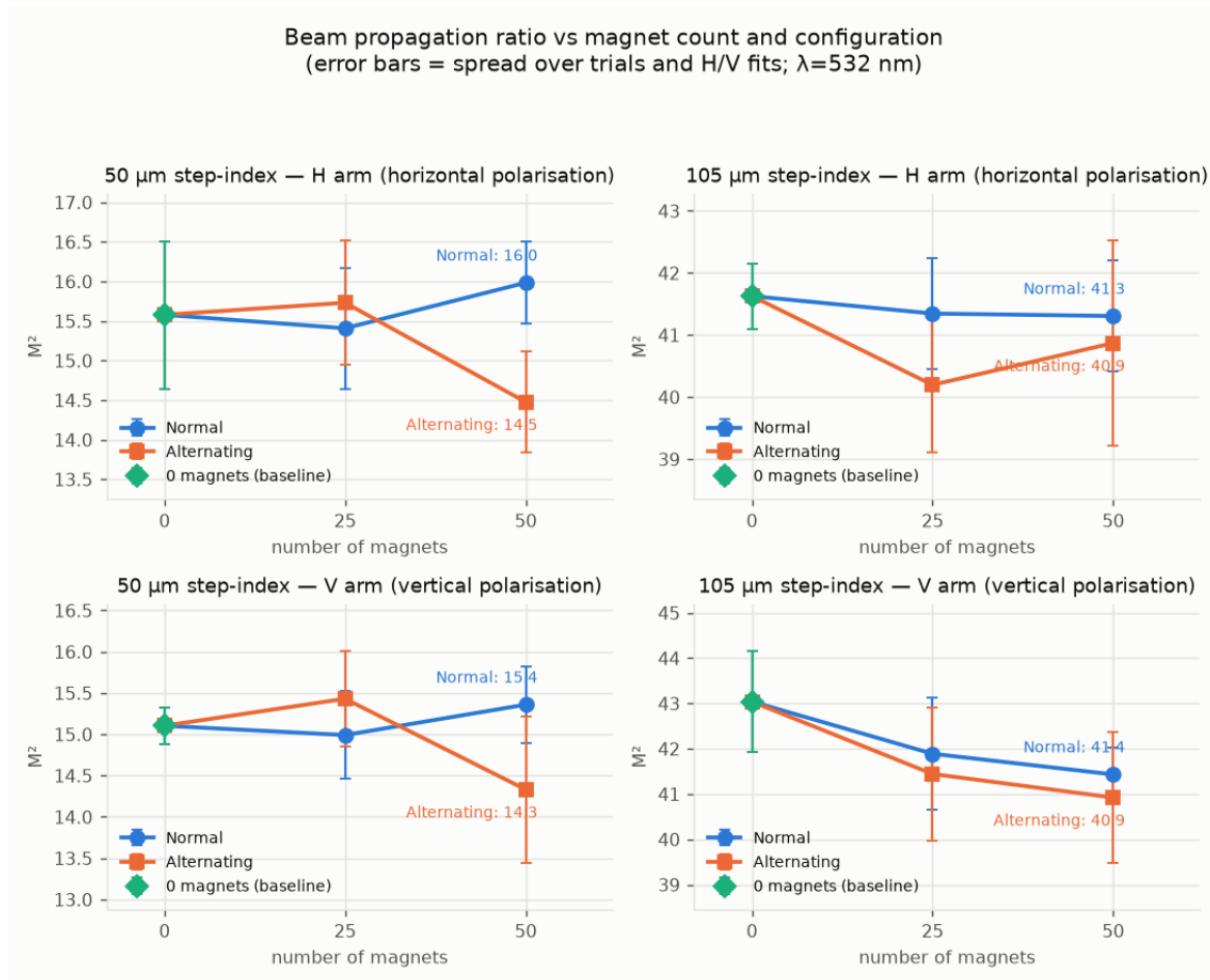
Figure 4. Absolute M^2 against magnet count, split by fibre and by polarisation arm, with the uniform (“Normal”) and alternating configurations overlaid. The 0-magnet baseline is shared by both configurations. The vertical scale spans only a few units of M^2 in every panel: on the scale of the baseline difference between the two fibres, all of these traces would be flat lines.
