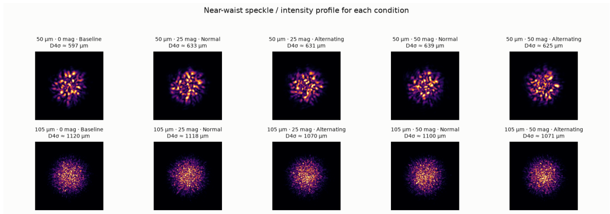
Figure 6. The near-waist intensity pattern for each condition, cropped to the beam and stretched to the 99.5th percentile. The 105 \mu\text{m} fibre carries visibly finer and far more numerous speckle grains than the 50 \mu\text{m} fibre — a direct visual counterpart of the mode counts in Section 3. Within a row the patterns are of similar size and grain, which is the M^2 result stated visually.
