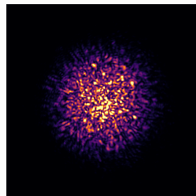
105 \mu\text{m} · 50 mag · Alternating D4\sigma \approx 1071 \mu\text{m}
