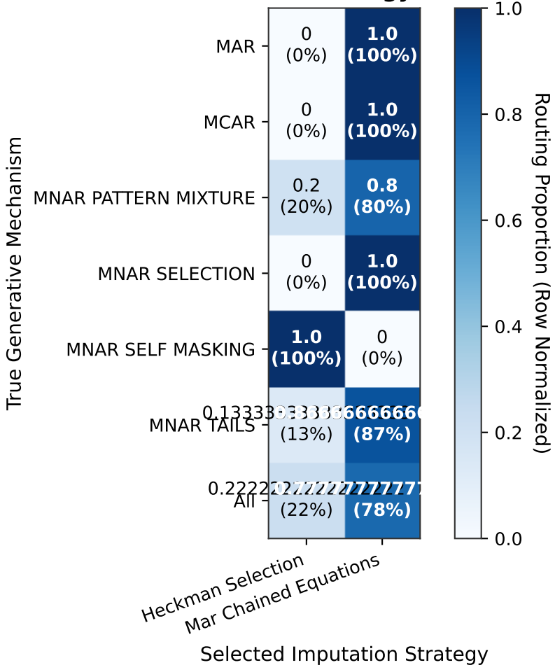
Figure 4: Umbra Auto-Router Strategy Selection Confusion Matrix
